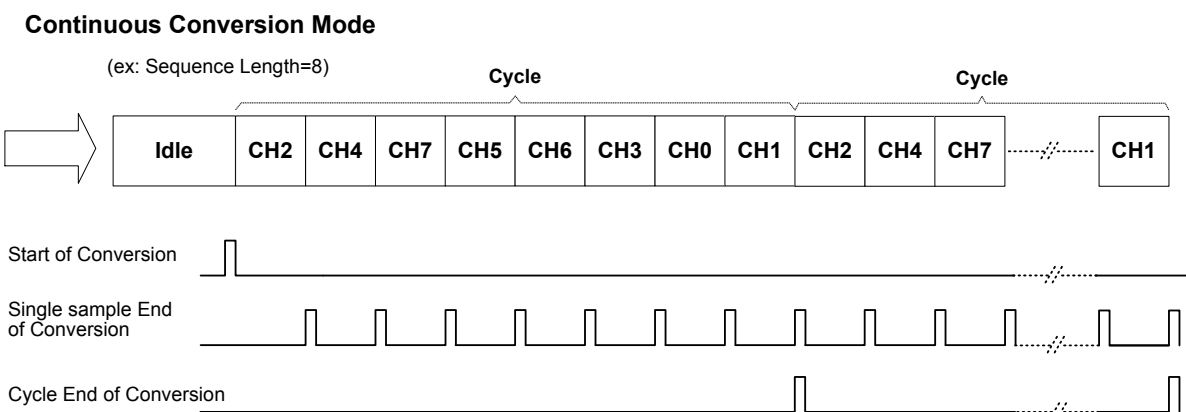
Figure 29. Continuous Conversion Mode
