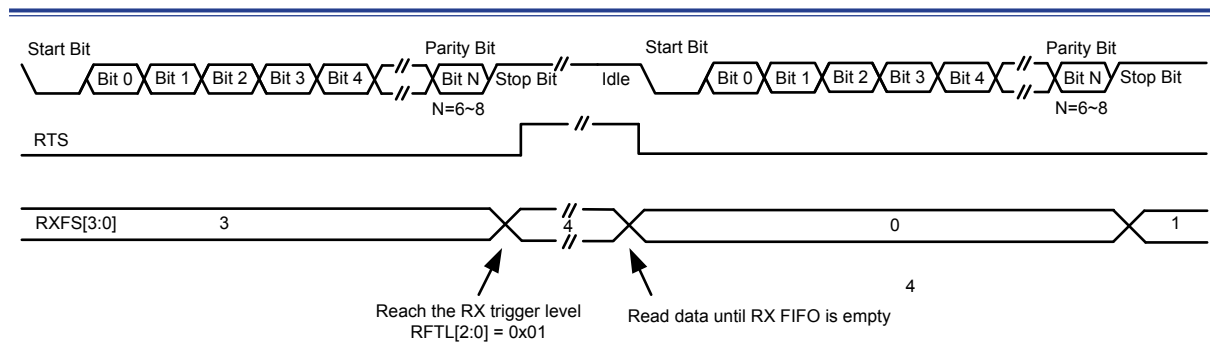
Figure 160. USART RTS Flow Control
