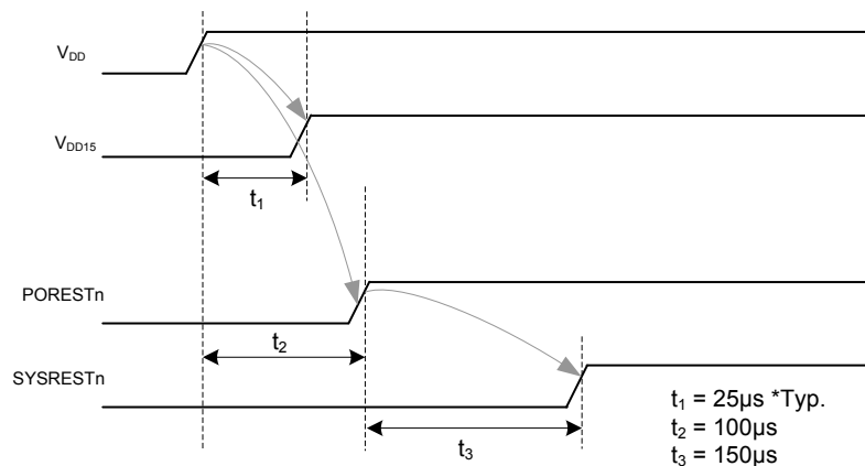
Figure 19. Power On Reset Sequence
