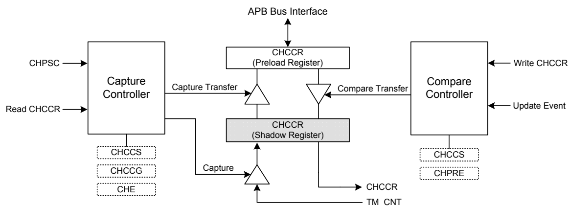
Figure 120. Capture/Compare Block Diagram
