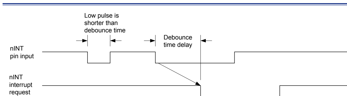
Figure 26. EXTI Interrupt Debounce Function
