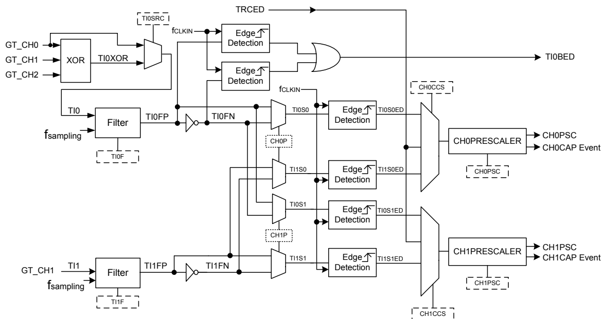
Figure 46. Channel 0 and Channel 1 Input Stages
