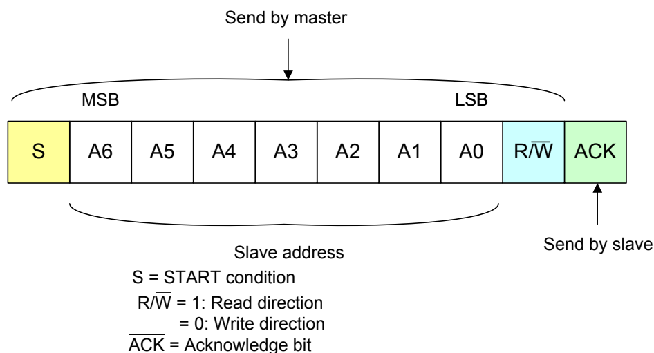
Figure 135. 7-bit Addressing Mode
