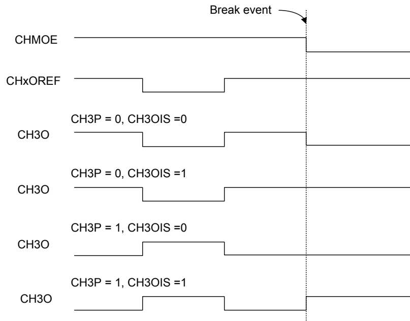
Figure 97. Channel 3 Output with a Break Event Occurrence
