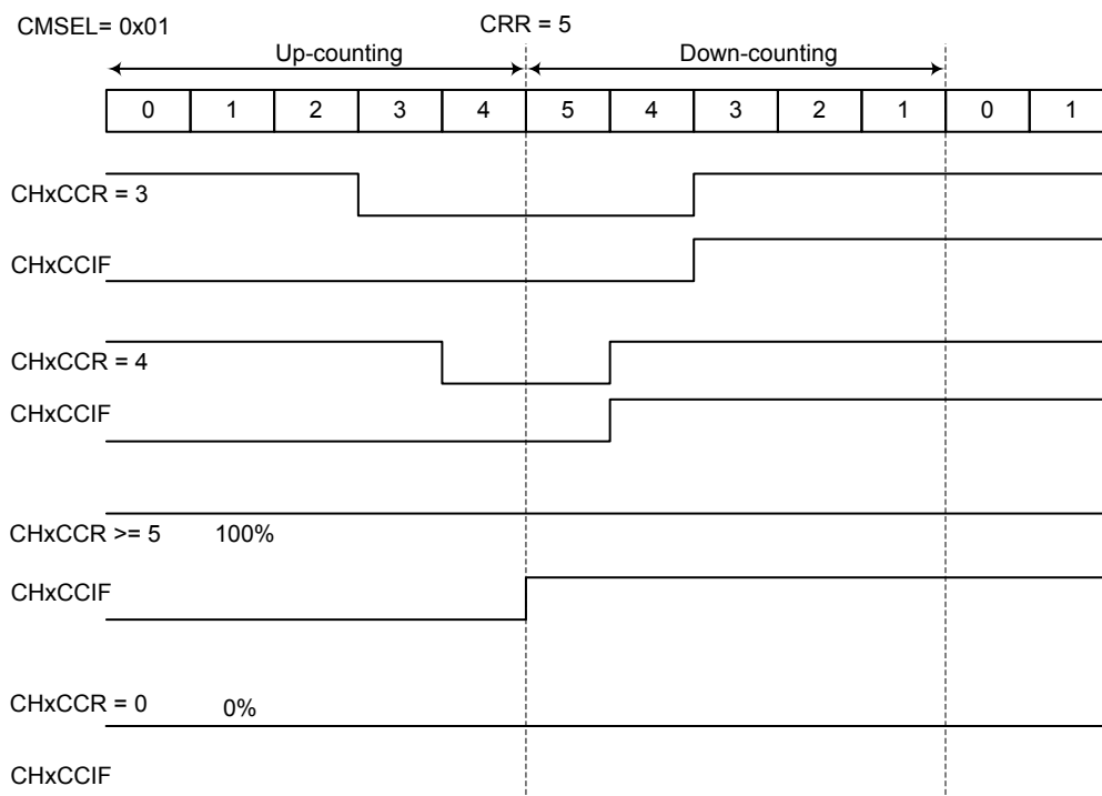
Figure 56. PWM Mode Channel Output Reference Signal and Counter in Center-align Mode
