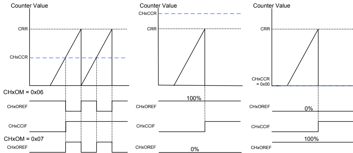
Figure 91. PWM Mode Channel Output Reference Signal and Counter in Up-counting Mode
