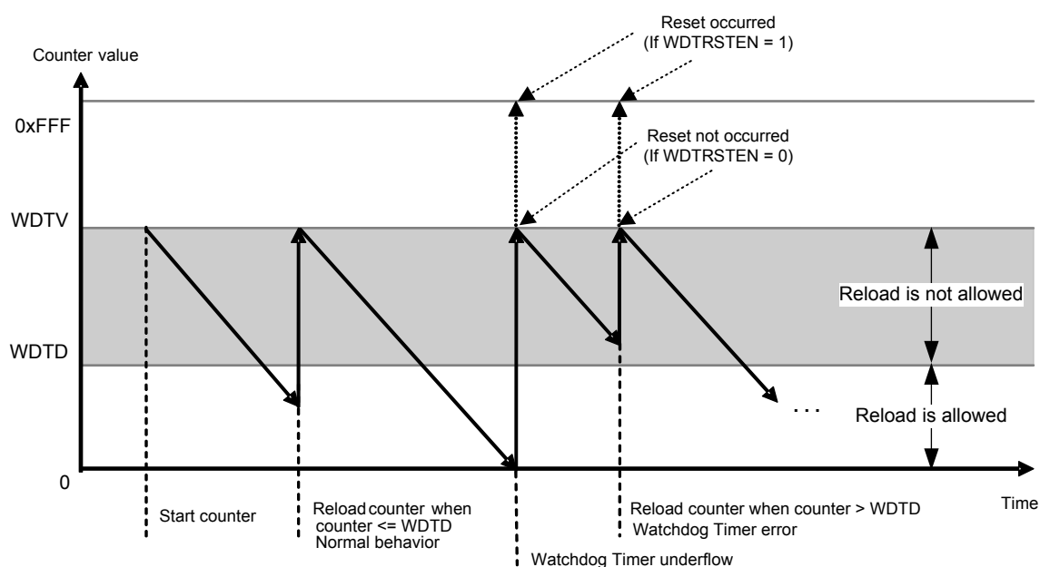
Figure 131. Watchdog Timer Behavior
