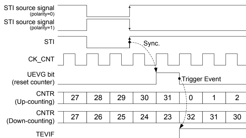
Figure 38. GPTM in Restart Mode
