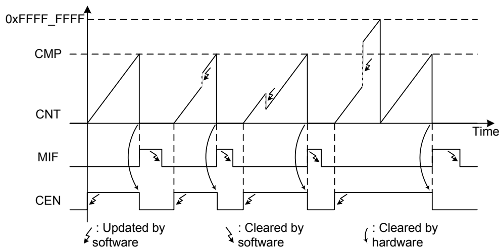
Figure 68. BFTM – One Shot Mode Counter Updating
