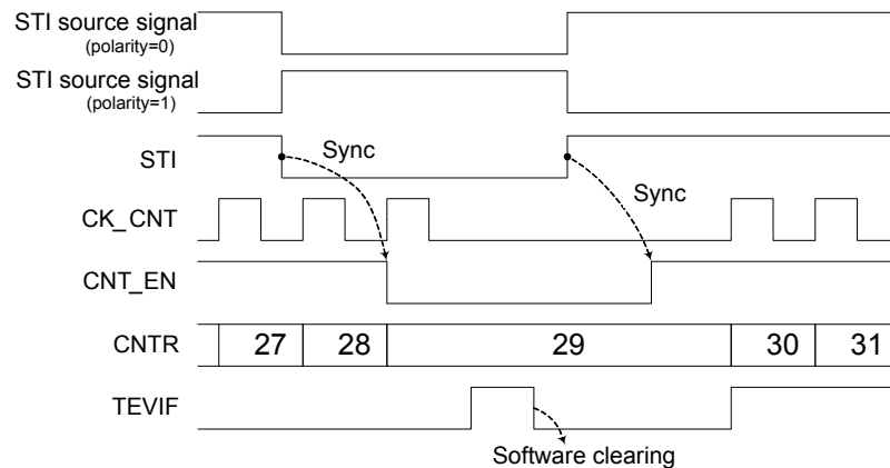
Figure 78. MCTM in Pause Mode
