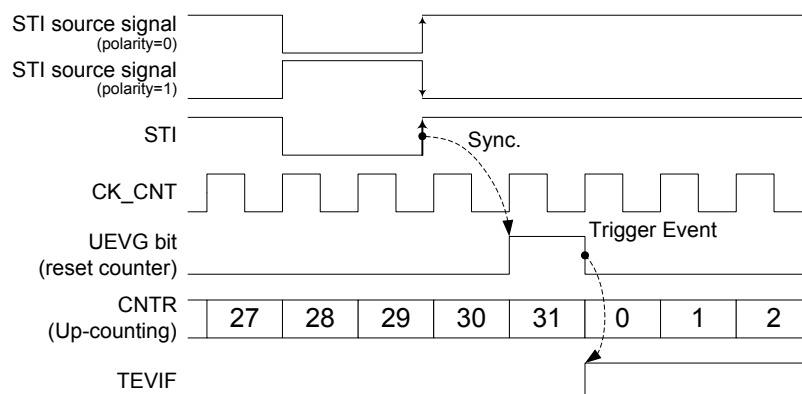
Figure 117. SCTM in Restart Mode
