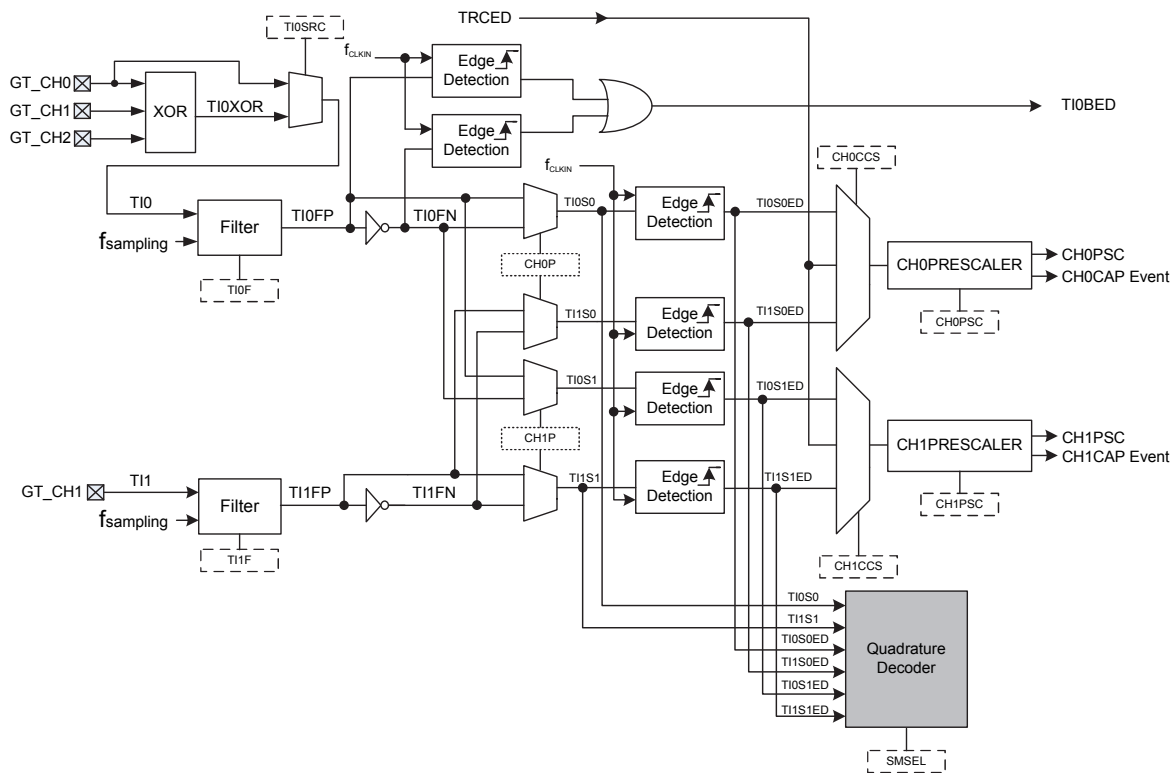
Figure 49. Input Stage and Quadrature Decoder Block Diagram
