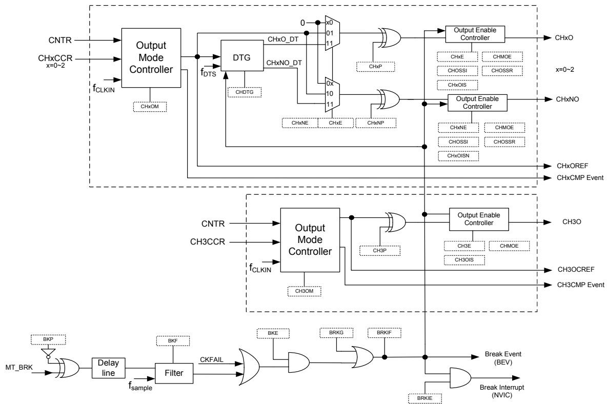
Figure 88. Output Stage Block Diagram
