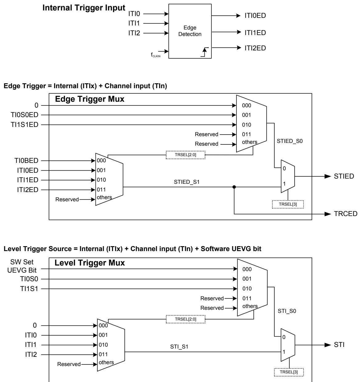
Figure 36. Trigger Control Block
