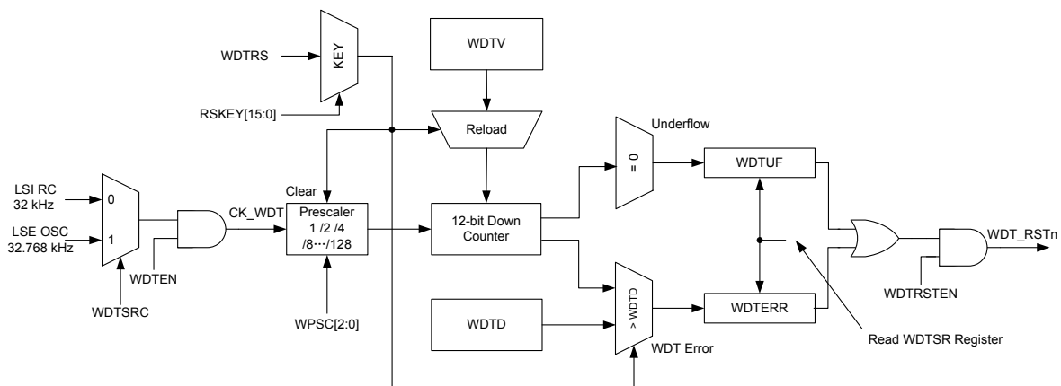
Figure 130. Watchdog Timer Block Diagram
