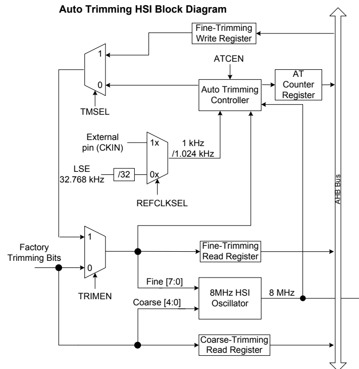
Figure 15. HSI Auto Trimming Block Diagram
