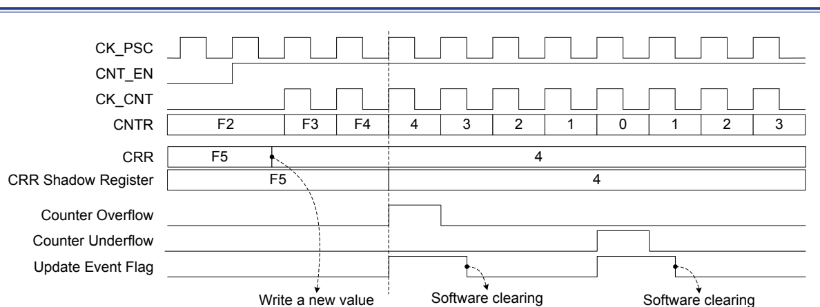
Figure 34. Center-aligned Counting Example
