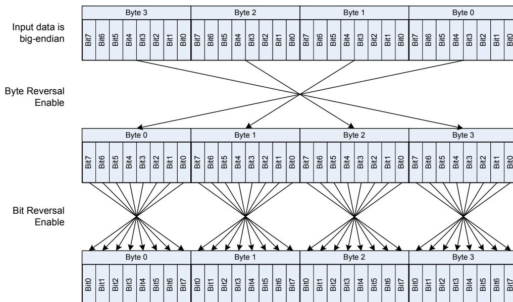
Figure 174. CRC Data Bit and Byte Reversal Example
