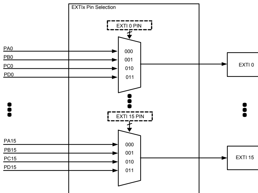
Figure 23. EXTI Channel Input Selection
