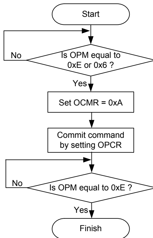
Figure 9. Mass Erase Operation Flowchart
