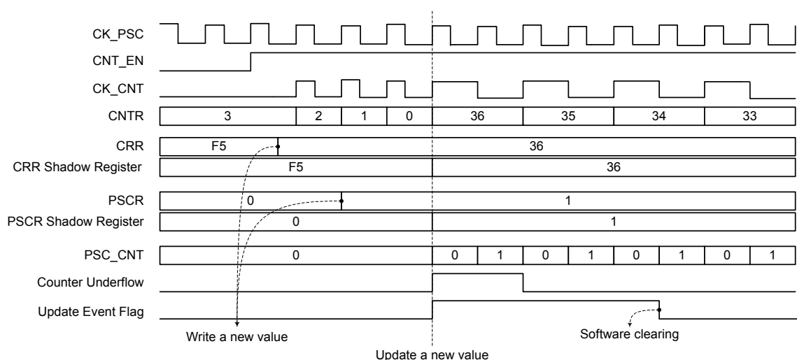
Figure 33. Down-counting Example
