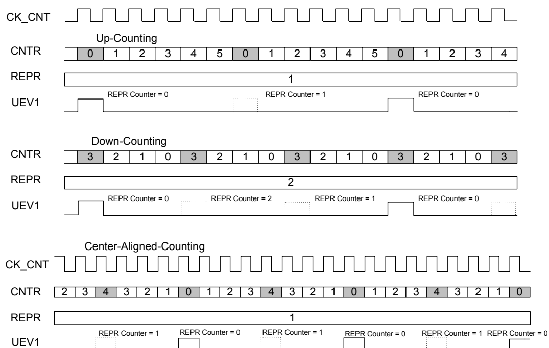
Figure 73. Update Event 1 Dependent Repetition Mechanism Example
