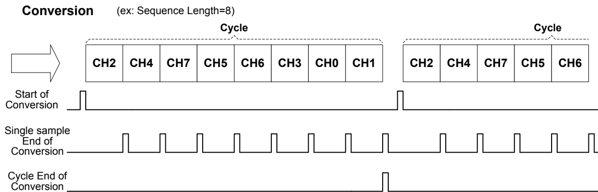
Figure 28. One Shot Conversion Mode
