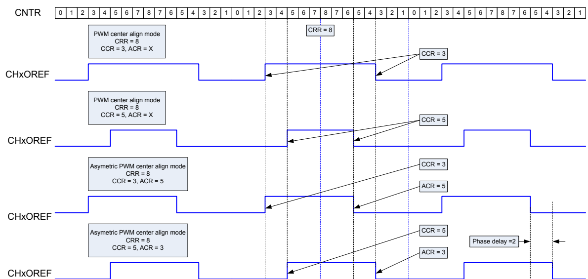
Figure 106. Asymmetric PWM Mode versus Center-aligned Counting Mode
