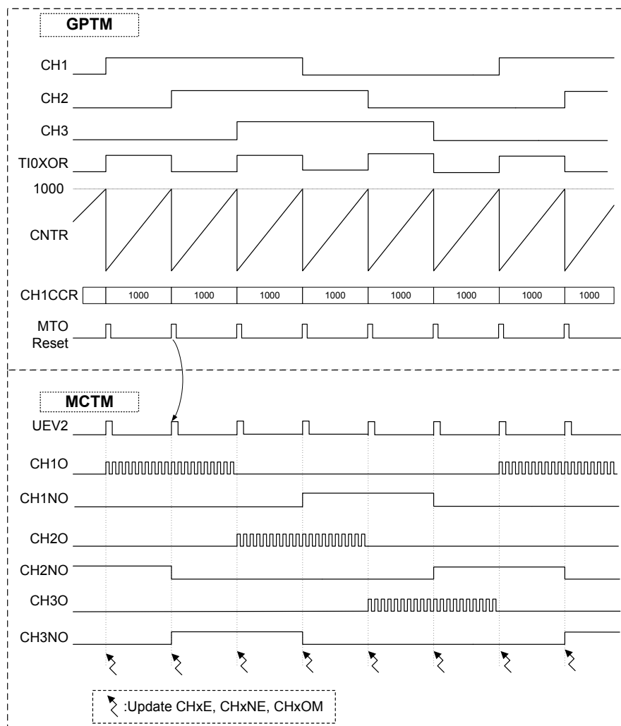
Figure 110. CH1XOR Input as Hall Sensor Interface
