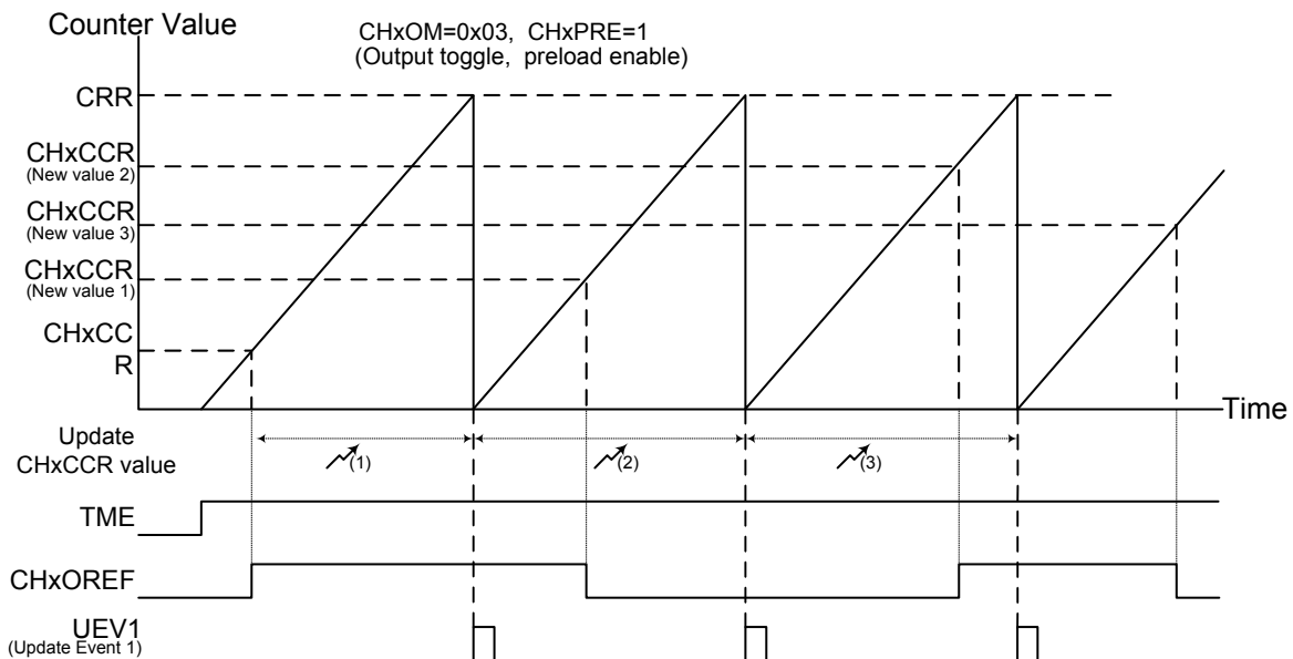
Figure 90. Toggle Mode Channel Output Reference Signal – CHxPRE = 1
