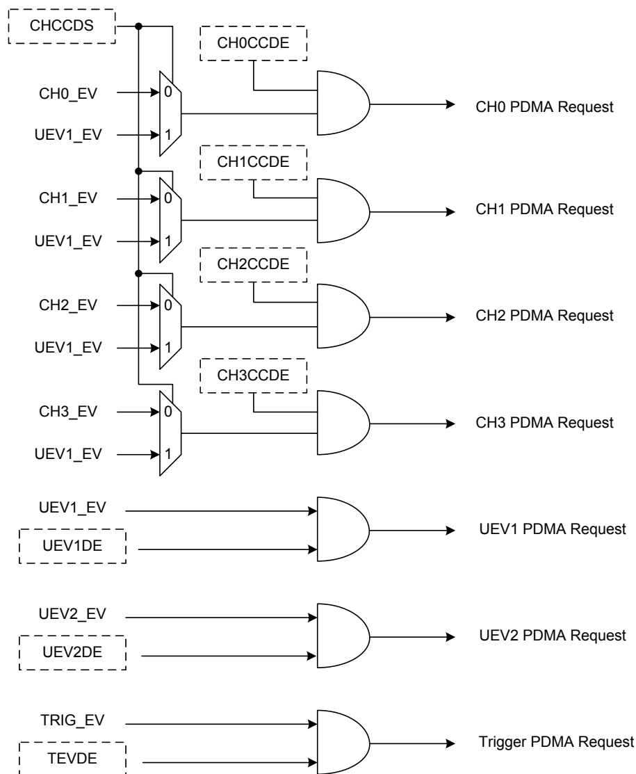
Figure 111. MCTM PDMA Mapping Diagram
