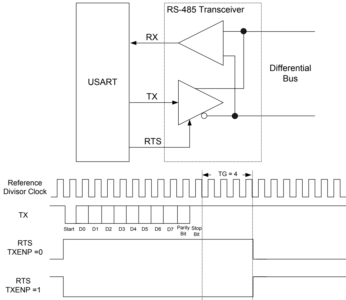
Figure 164. RS485 Interface and Waveform
