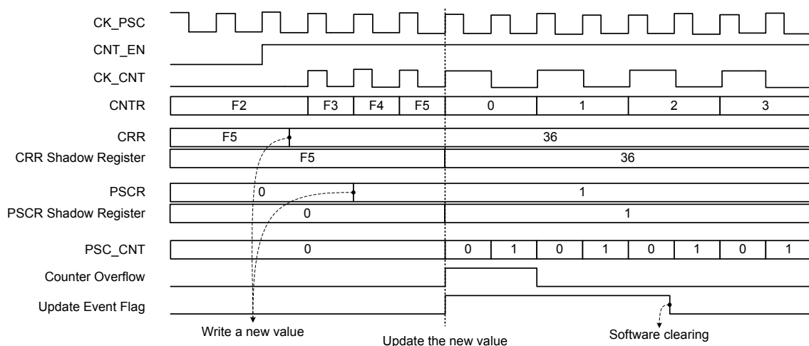
Figure 113. Up-counting Example
