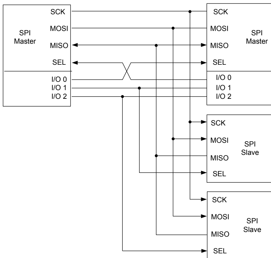
Figure 155. SPI Multi-Master Slave Environment
