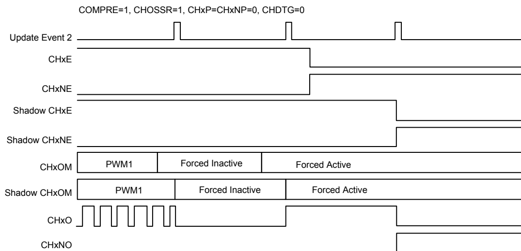
Figure 102. CHxE, CHxNE and CHxOM Updated by Update Event 2
