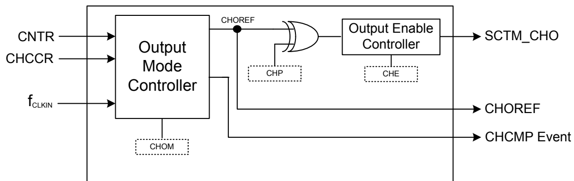
Figure 124. Output Stage Block Diagram
