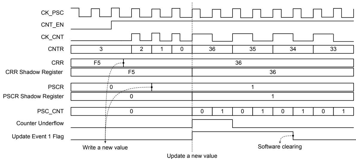
Figure 71. Down-counting Example
