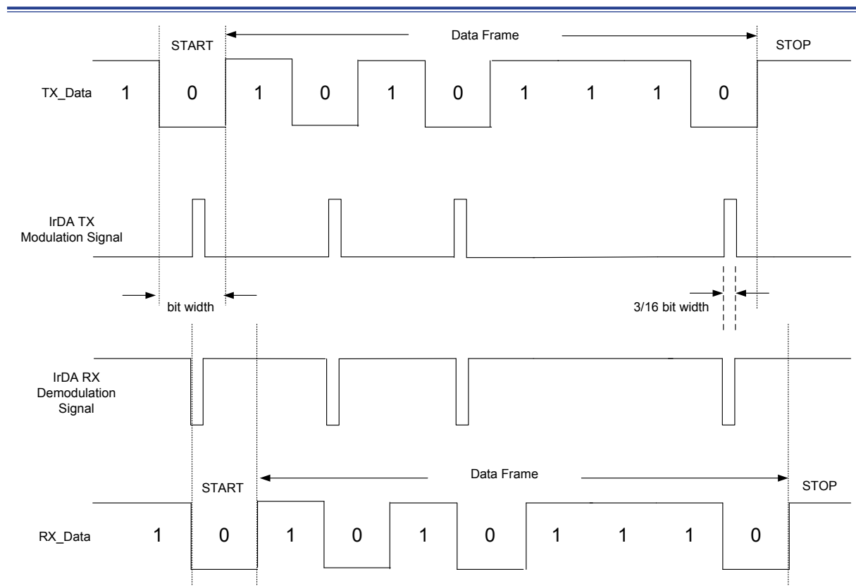
Figure 162. IrDA Modulation and Demodulation
