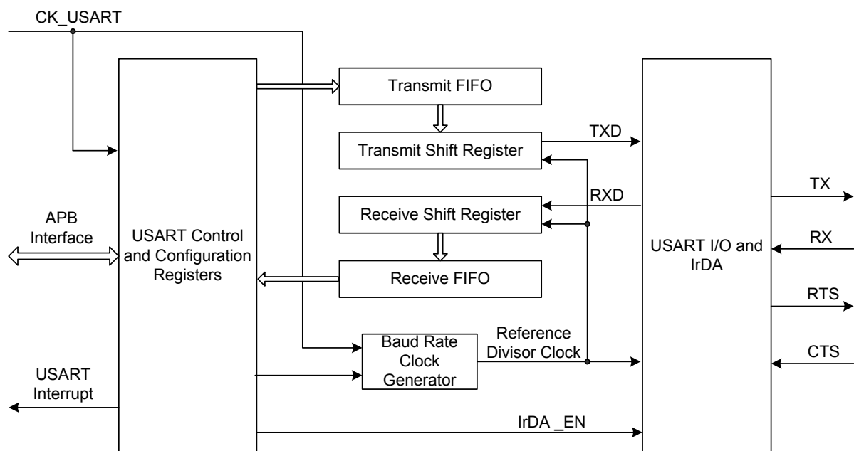
Figure 156. USART Block Diagram
