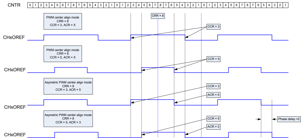
Figure 60. Asymmetric PWM Mode versus Center Align Counting Mode
