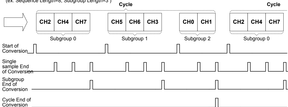
Figure 30. Discontinuous Conversion Mode
