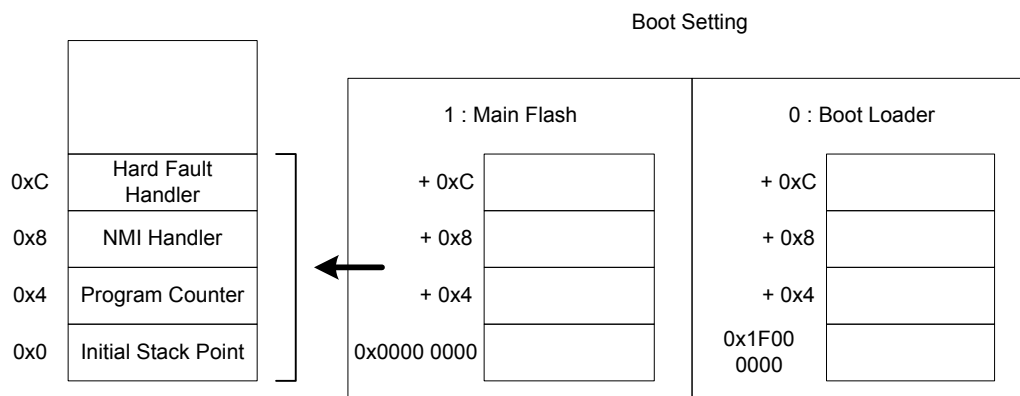
Figure 7. Vector Remapping
