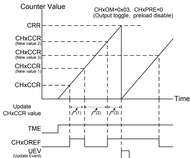
Figure 52. Toggle Mode Channel Output Reference Signal (CHxPRE = 0)
