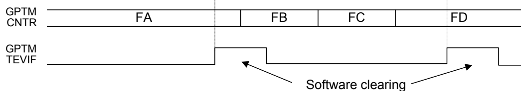
Figure 107. Pausing GPTM using the MCTM CH0OREF Signal
