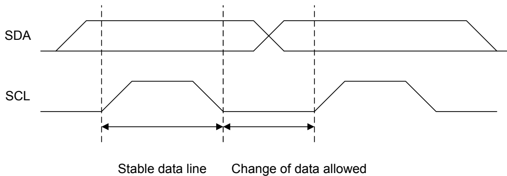
Figure 134. Data Validity
