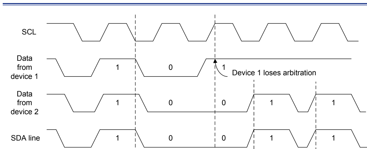
Figure 140. Two Master Arbitration Procedure
