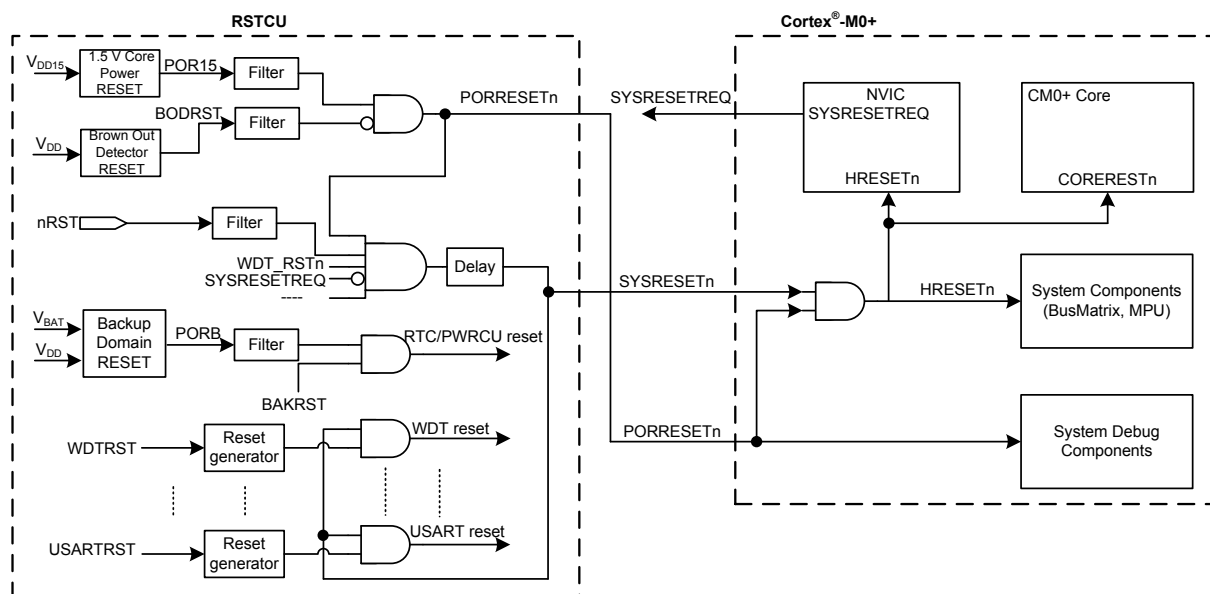
Figure 18. RSTCU Block Diagram
