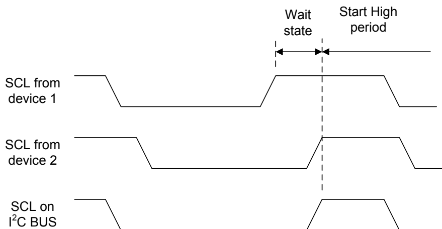
Figure 139. Clock Synchronization during Arbitration
