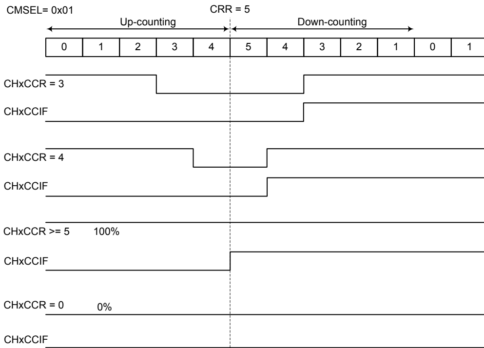
Figure 93. PWM Mode 1 Channel Output Reference Signal and Counter in Center-aligned Counting Mode
