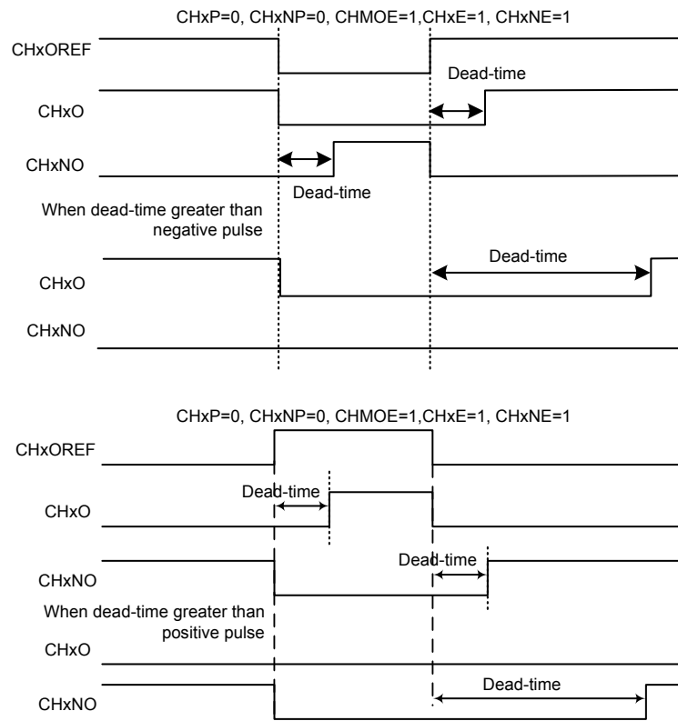
Figure 94. Dead-time Insertion Performed for Complementary Outputs
