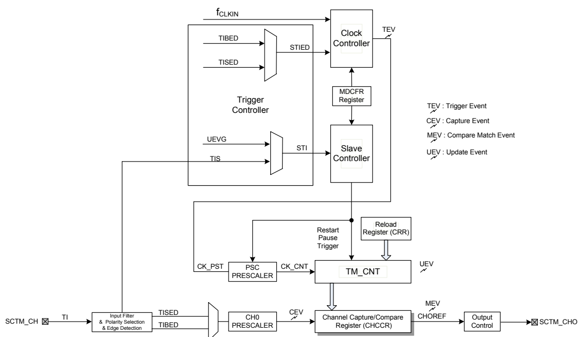
Figure 112. SCTM Block Diagram
