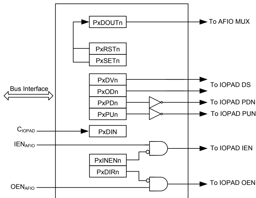
Figure 20. GPIO Block Diagram
