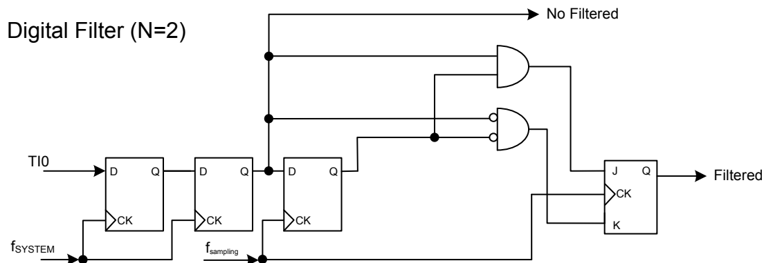
Figure 48. TI0 Digital Filter Diagram with N = 2
