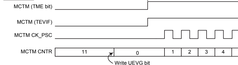
Figure 63. Trigger GPTM and MCTM with the GPTM CH0 Input
