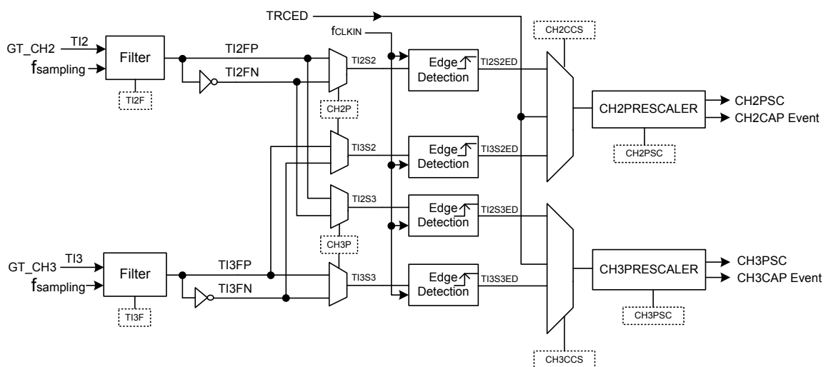
Figure 47. Channel 2 and Channel 3 Input Stages
