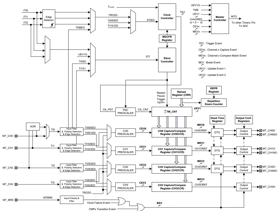
Figure 69. MCTM Block Diagram
