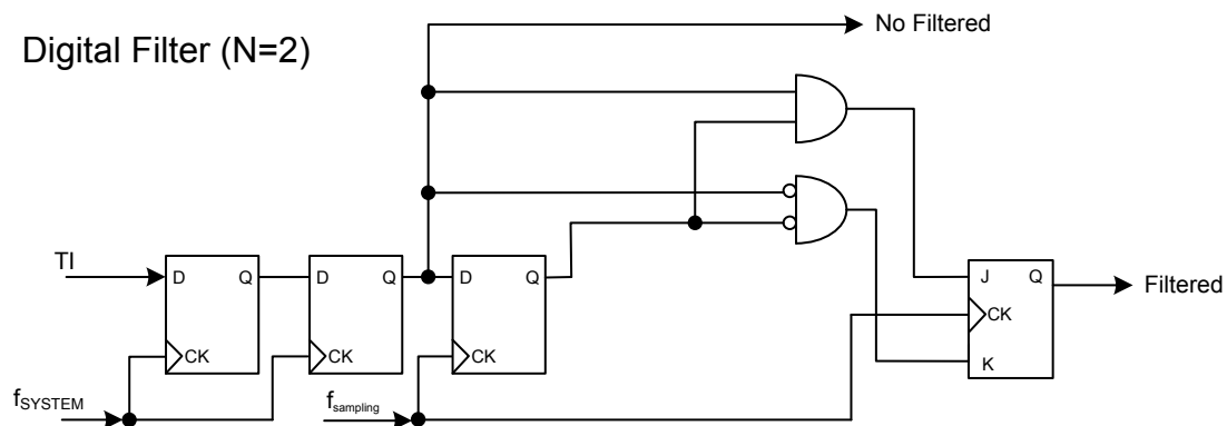
Figure 123. TI Digital Filter Diagram with N = 2
