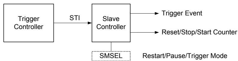
Figure 37. Slave Controller Diagram
