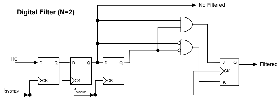
Figure 87. TIO Digital Filter Diagram with N = 2
