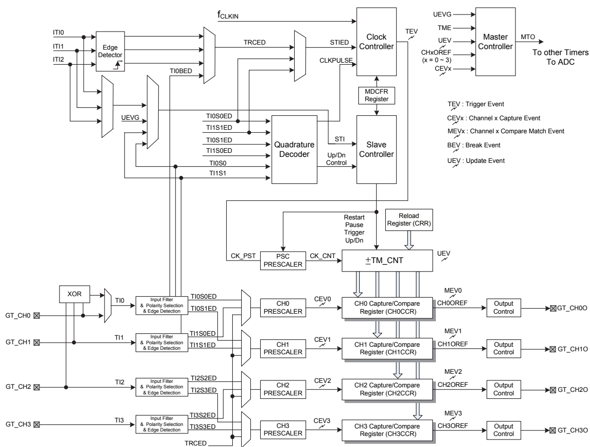
Figure 31. GPTM Block Diagram
