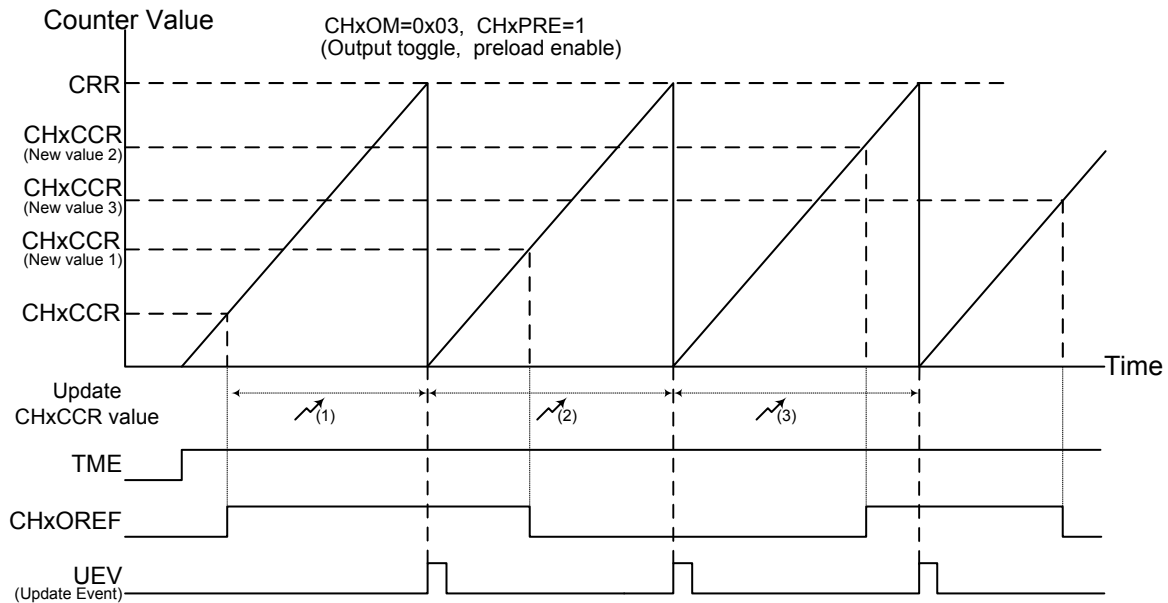
Figure 53. Toggle Mode Channel Output Reference Signal (CHxPRE = 1)
