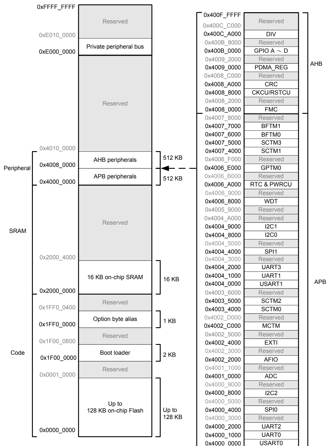
Figure 4. Memory Map
