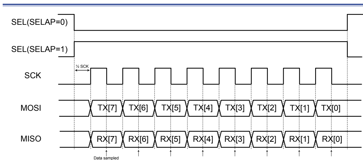
Figure 149. SPI Single Byte Transfer Timing Diagram – CPOL = 0, CPHA = 1
