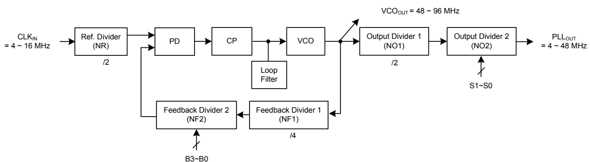
Figure 16. PLL Block Diagram
