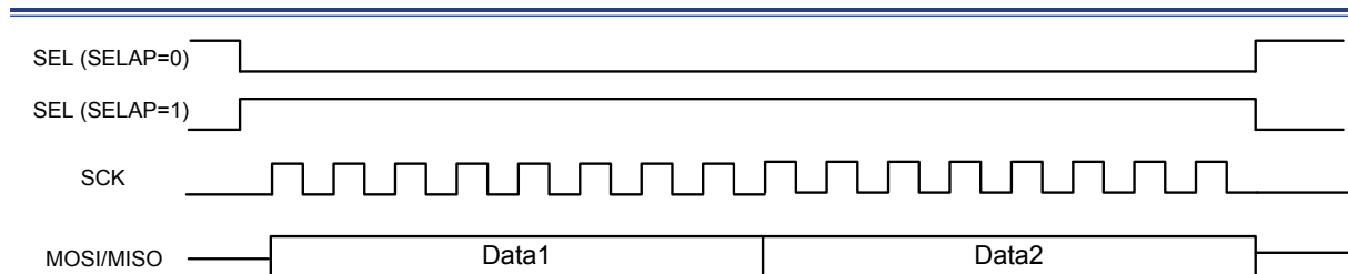
Figure 150. SPI Continuous Transfer Timing Diagram – CPOL = 0, CPHA = 1
