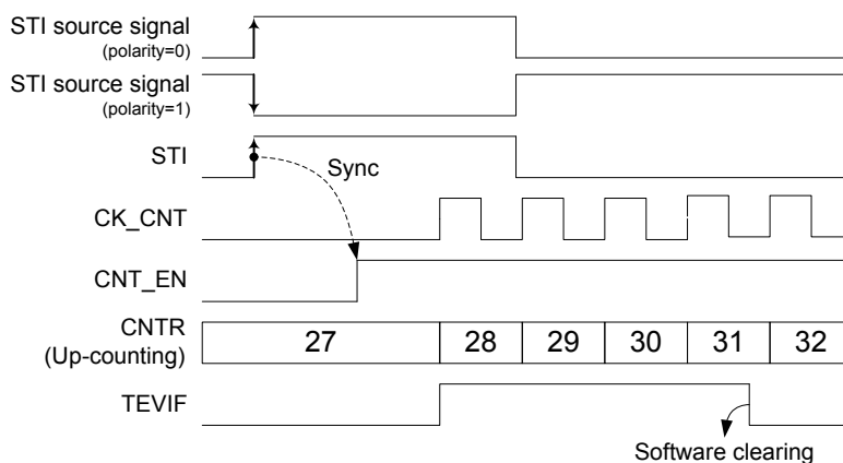
Figure 119. SCTM in Trigger Mode
