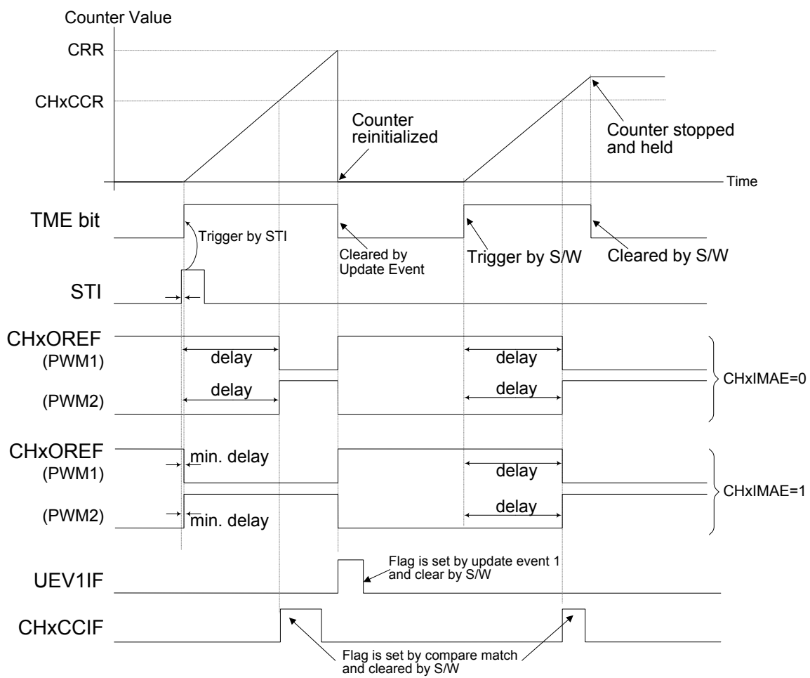
Figure 104. Single Pulse Mode
