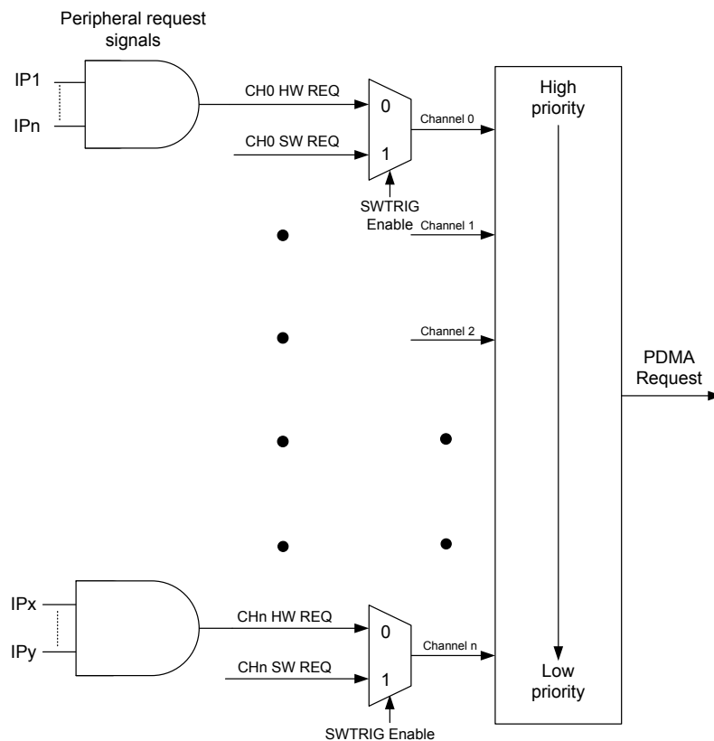
Figure 171. PDMA Request Mapping Architecture
