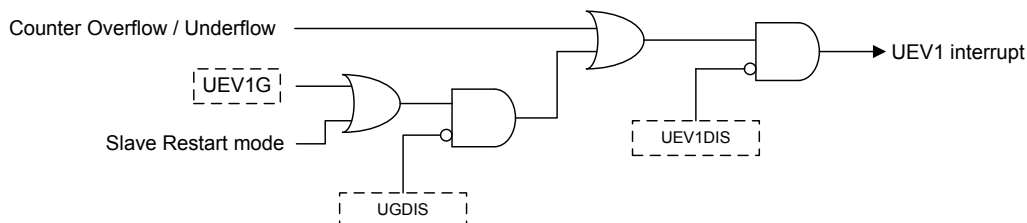
Figure 101. Update Event 1 Setup Diagram
