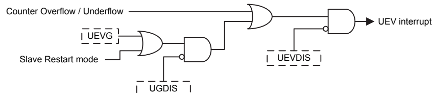
Figure 57. Update Event Setting Diagram
