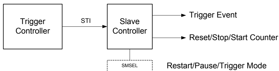
Figure 76. Slave Controller Diagram
