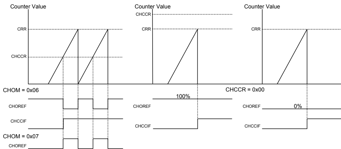
Figure 127. PWM Mode Channel Output Reference Signal
