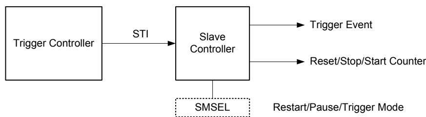
Figure 116. Slave Controller Diagram
