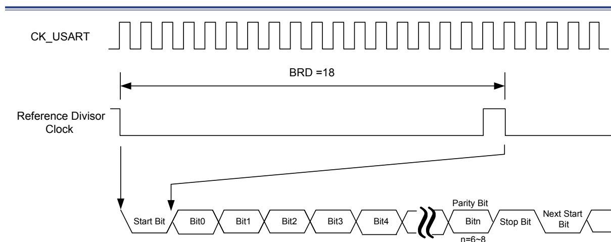
Figure 158. USART Clock CK_USART and Data Frame Timing
