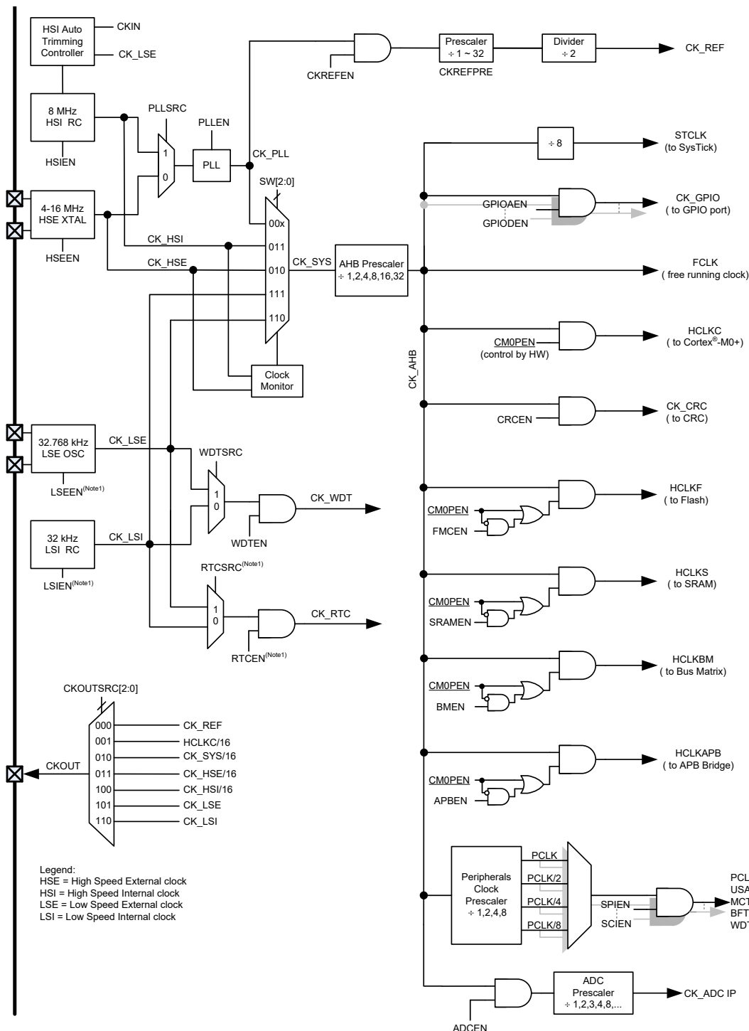
Figure 13. CKCU Block Diagram
