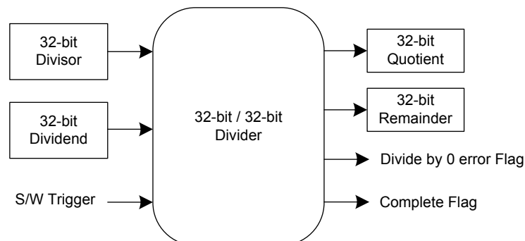
Figure 175. Divider Functional Diagram
