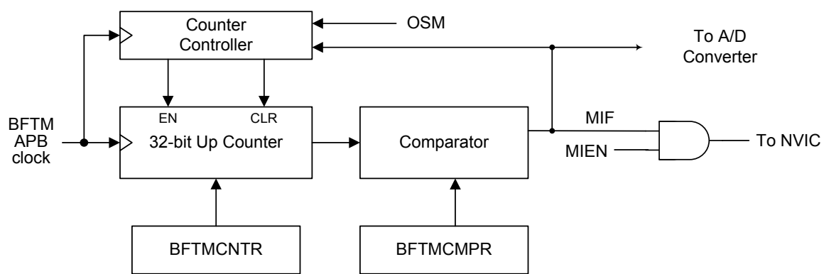
Figure 65. BFTM Block Diagram
