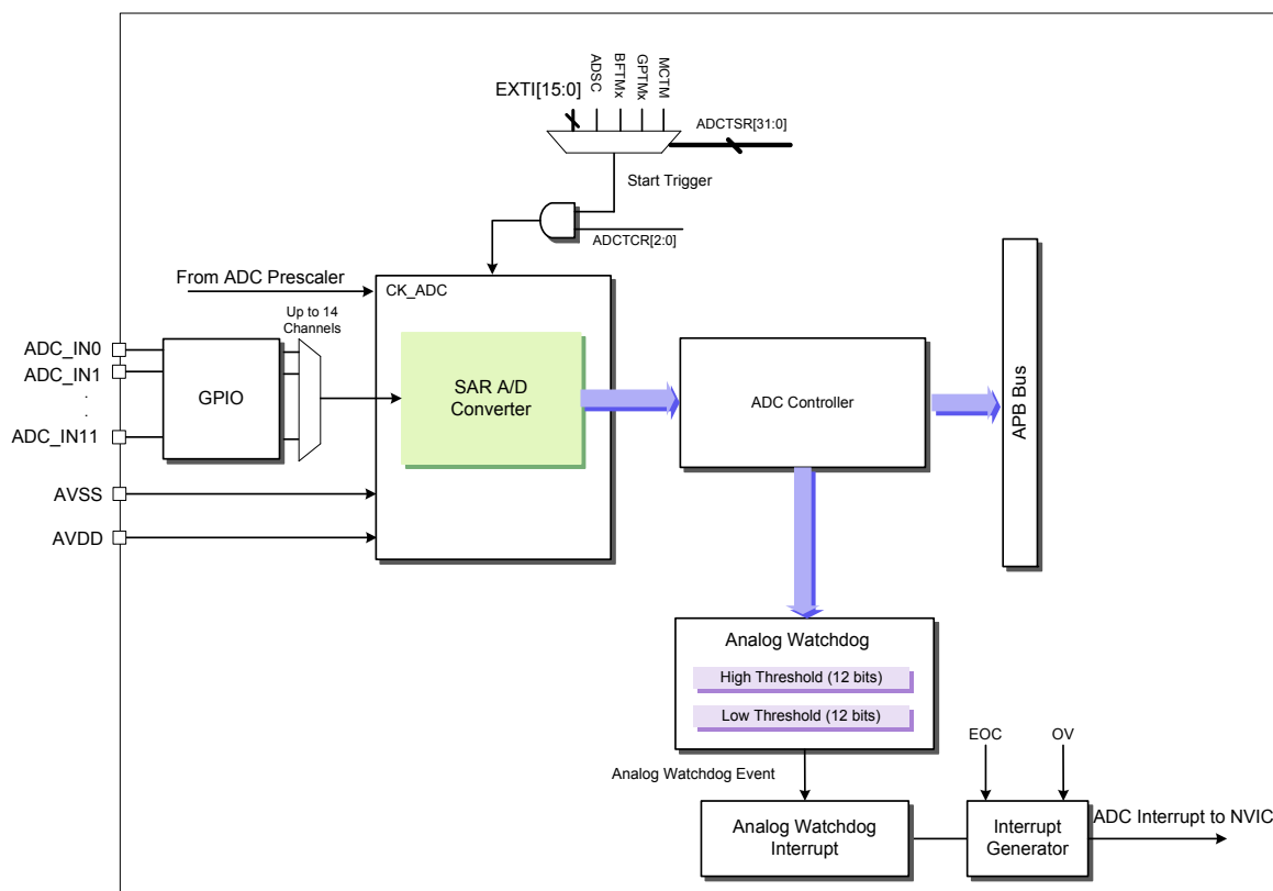
Figure 27. ADC Block Diagram
