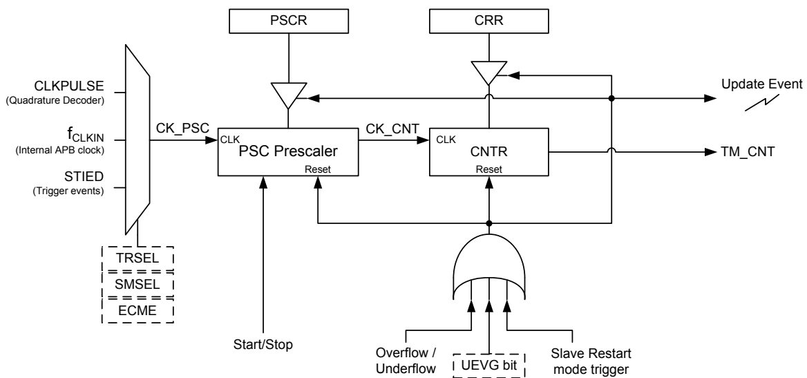
Figure 35. GPTM Clock Selection Source
