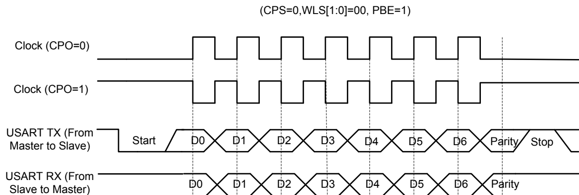
Figure 166. 8-bit Format USART Synchronous Waveform
