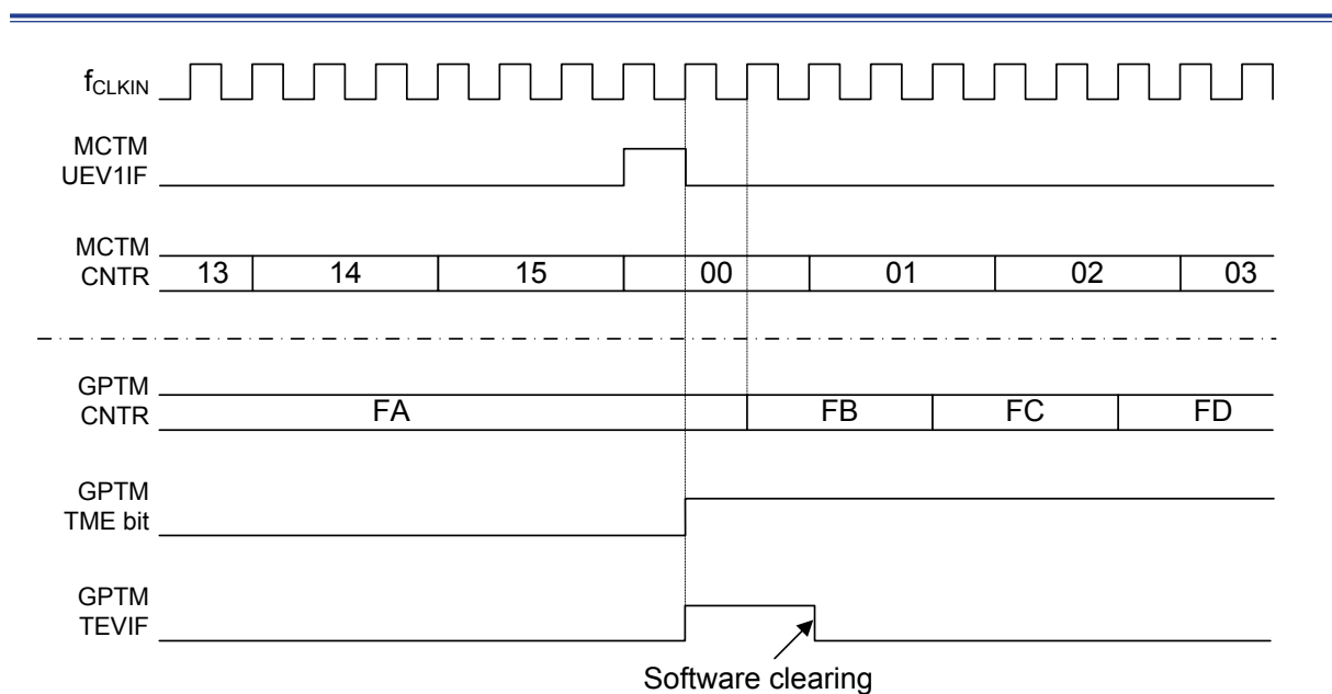
Figure 108. Triggering GPTM with MCTM Update Event 1
