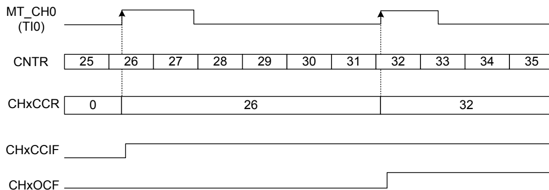
Figure 83. Input Capture Mode
