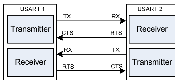
Figure 159. Hardware Flow Control between 2 USARTs
