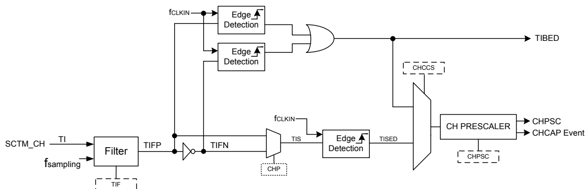
Figure 122. Channel Input Stages
