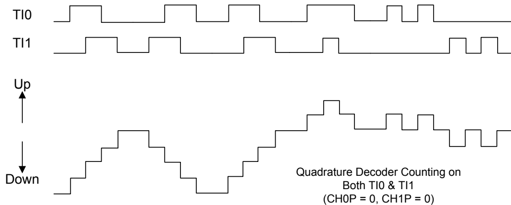
Figure 50. Both TI0 and TI1 Quadrature Decoder Counting
