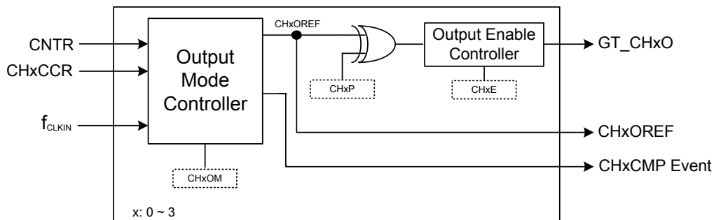
Figure 51. Output Stage Block Diagram
