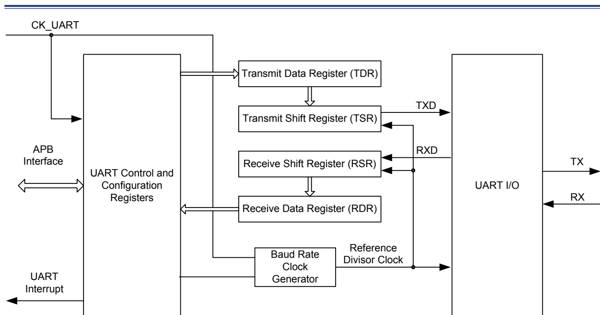
Figure 167. UART Block Diagram
