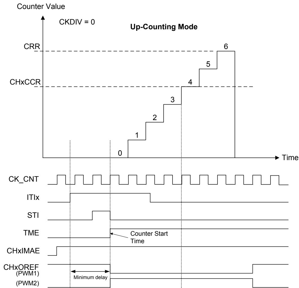
Figure 59. Immediate Active Mode Minimum Delay
