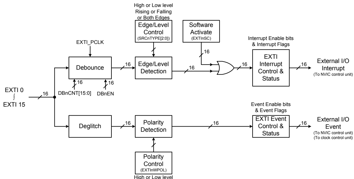
Figure 24. EXTI Block Diagram
