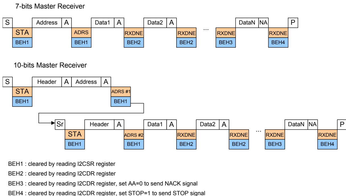
Figure 142. Master Receiver Timing Diagram
