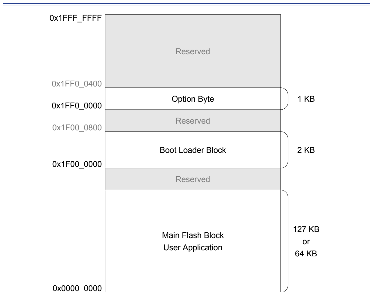
Figure 6. Flash Memory Map
