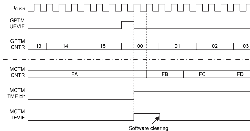
Figure 62. Triggering MCTM with GPTM Update Event
