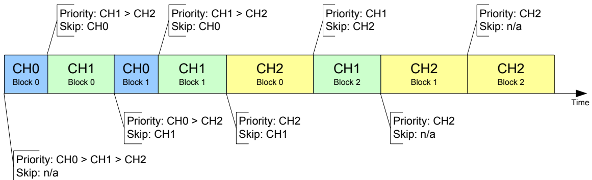
Figure 172. PDMA Channel Arbitration and Scheduling Example
