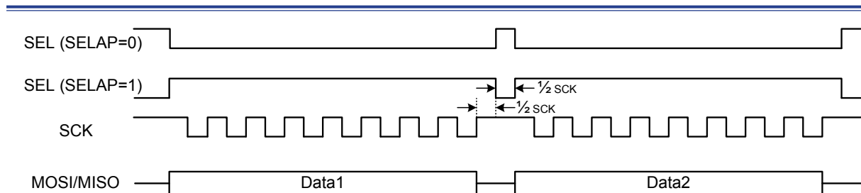
Figure 152. SPI Continuous Transfer Timing Diagram – CPOL = 1, CPHA = 0
