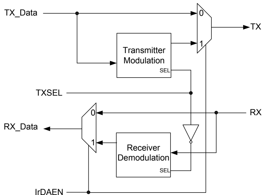
Figure 163. USART I/O and IrDA Block Diagram
