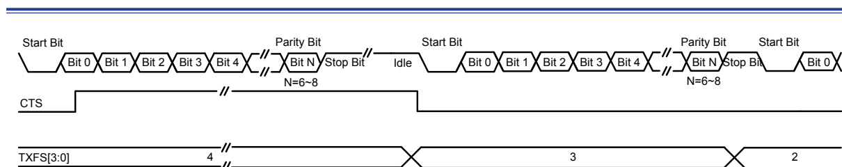
Figure 161. USART CTS Flow Control
