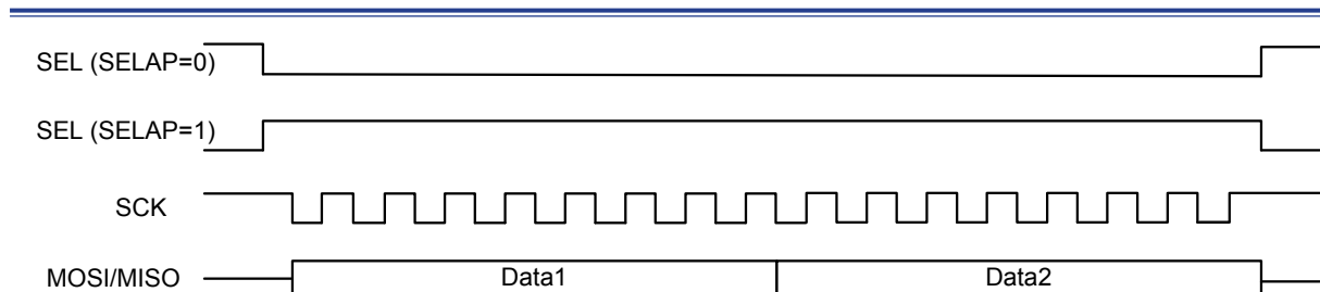
Figure 154. SPI Continuous Transfer Timing Diagram – CPOL = 1, CPHA = 1
