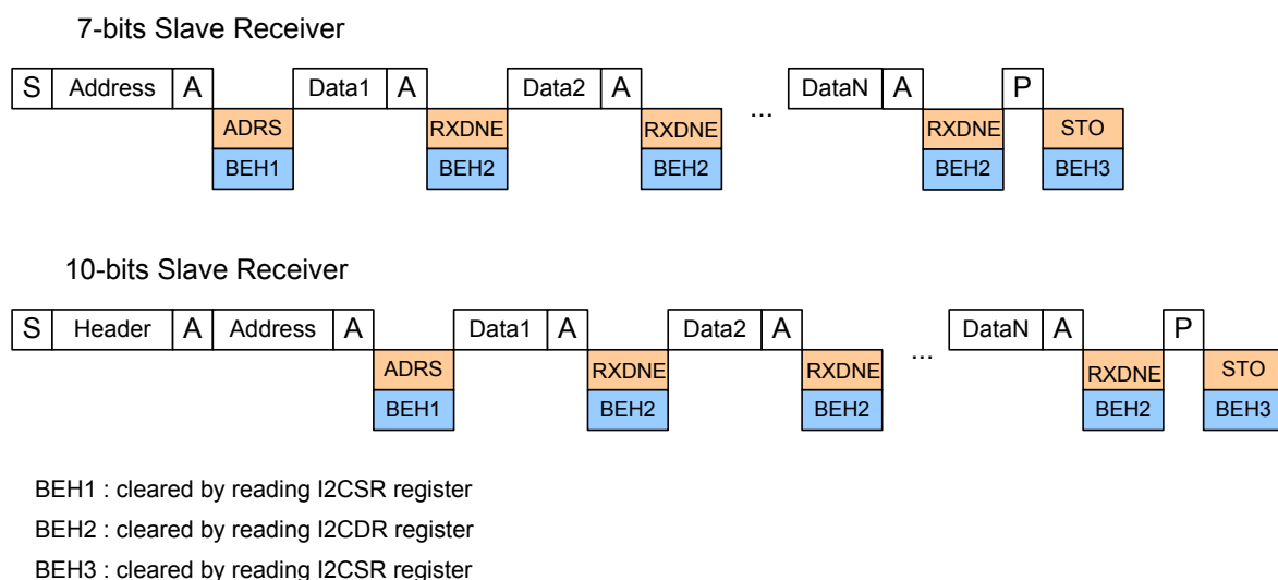
Figure 144. Slave Receiver Timing Diagram
