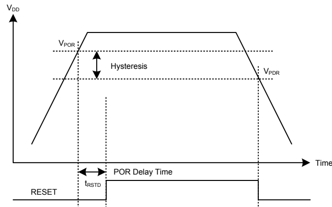
Figure 12. Power On Reset / Power Down Reset Waveform
