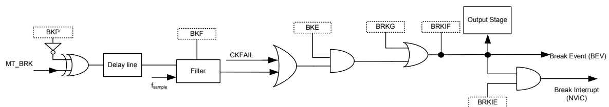
Figure 95. MCTM Break Signal Block Diagram
