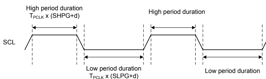
Figure 145. SCL Timing Diagram
