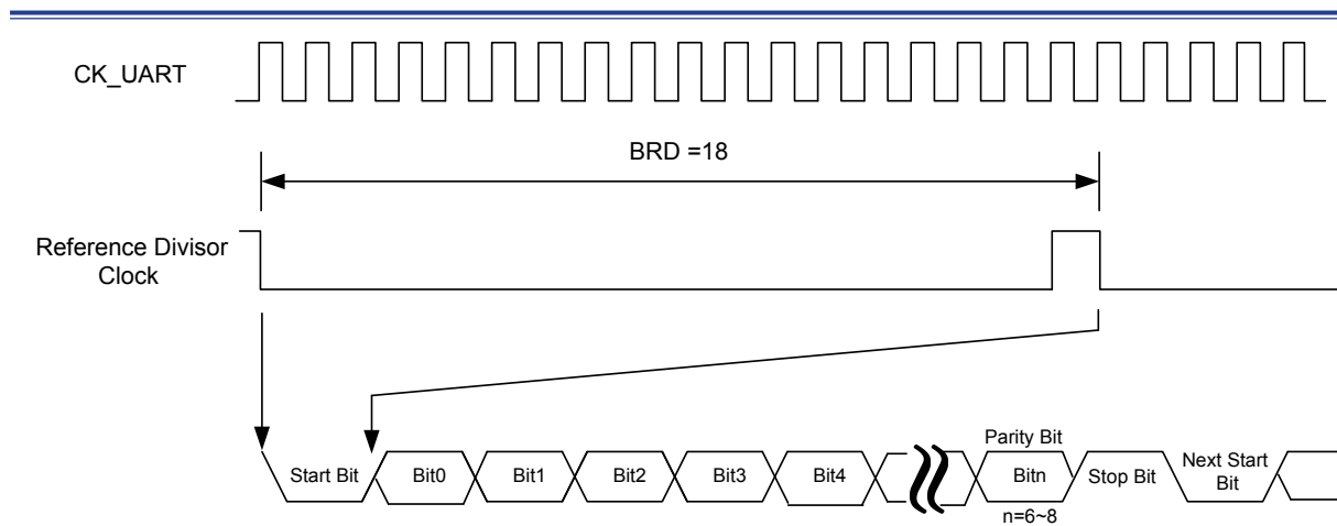
Figure 169. UART Clock CK_UART and Data Frame Timing
