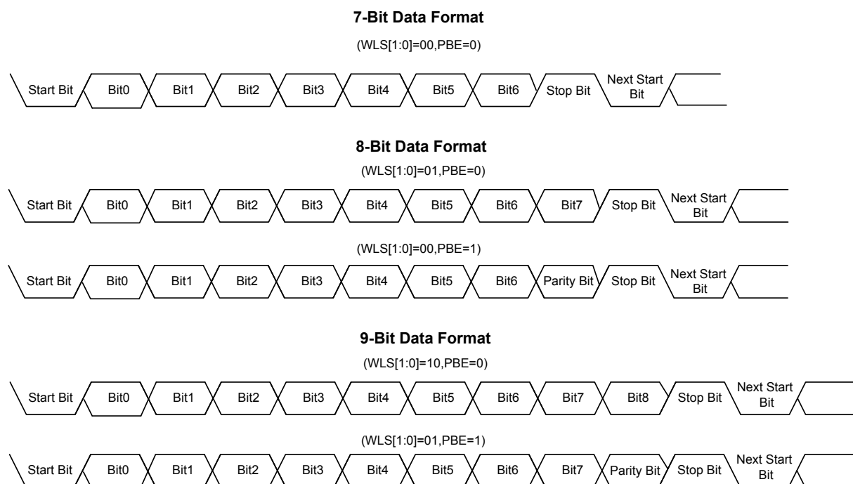
Figure 168. UART Serial Data Format
