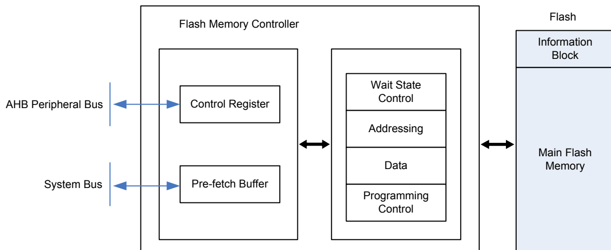
Figure 5. Flash Memory Controller Block Diagram
