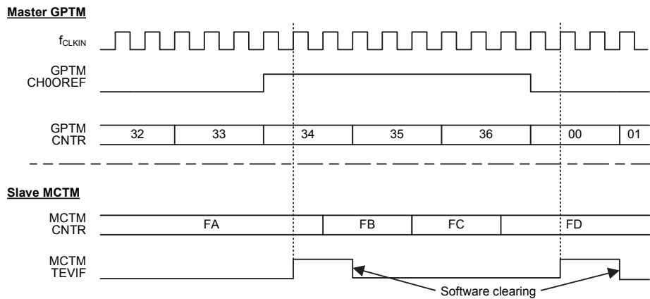
Figure 61. Pausing MCTM using the GPTM CH0OREF Signal
