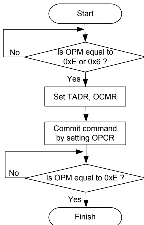
Figure 8. Page Erase Operation Flowchart
