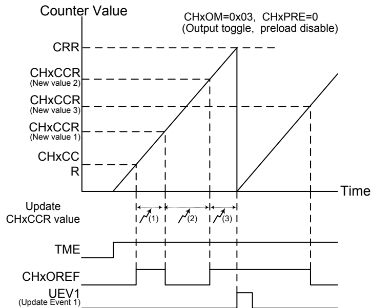
Figure 89. Toggle Mode Channel Output Reference Signal – CHxPRE = 0
