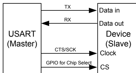
Figure 165. USART Synchronous Transmission Example
