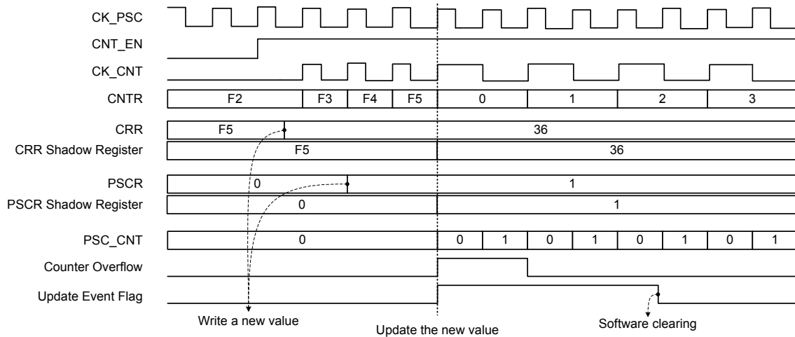
Figure 32. Up-counting Example
