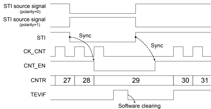
Figure 118. SCTM in Pause Mode
