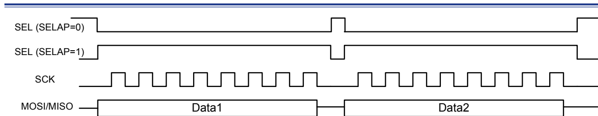
Figure 148. SPI Continuous Data Transfer Timing Diagram – CPOL = 0, CPHA = 0
