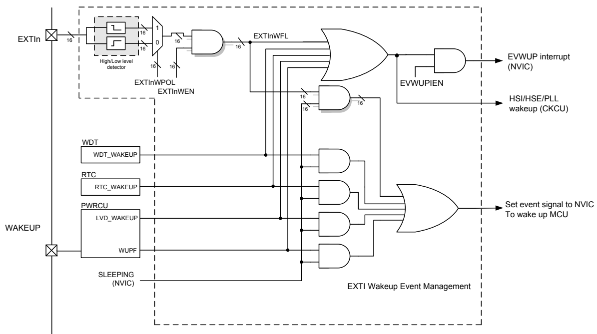
Figure 25. EXTI Wake-up Event Management
