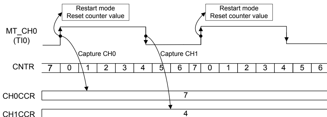
Figure 84. PWM Pulse Width Measurement Example
