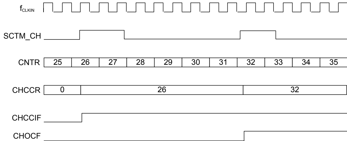
Figure 121. Input Capture Mode
