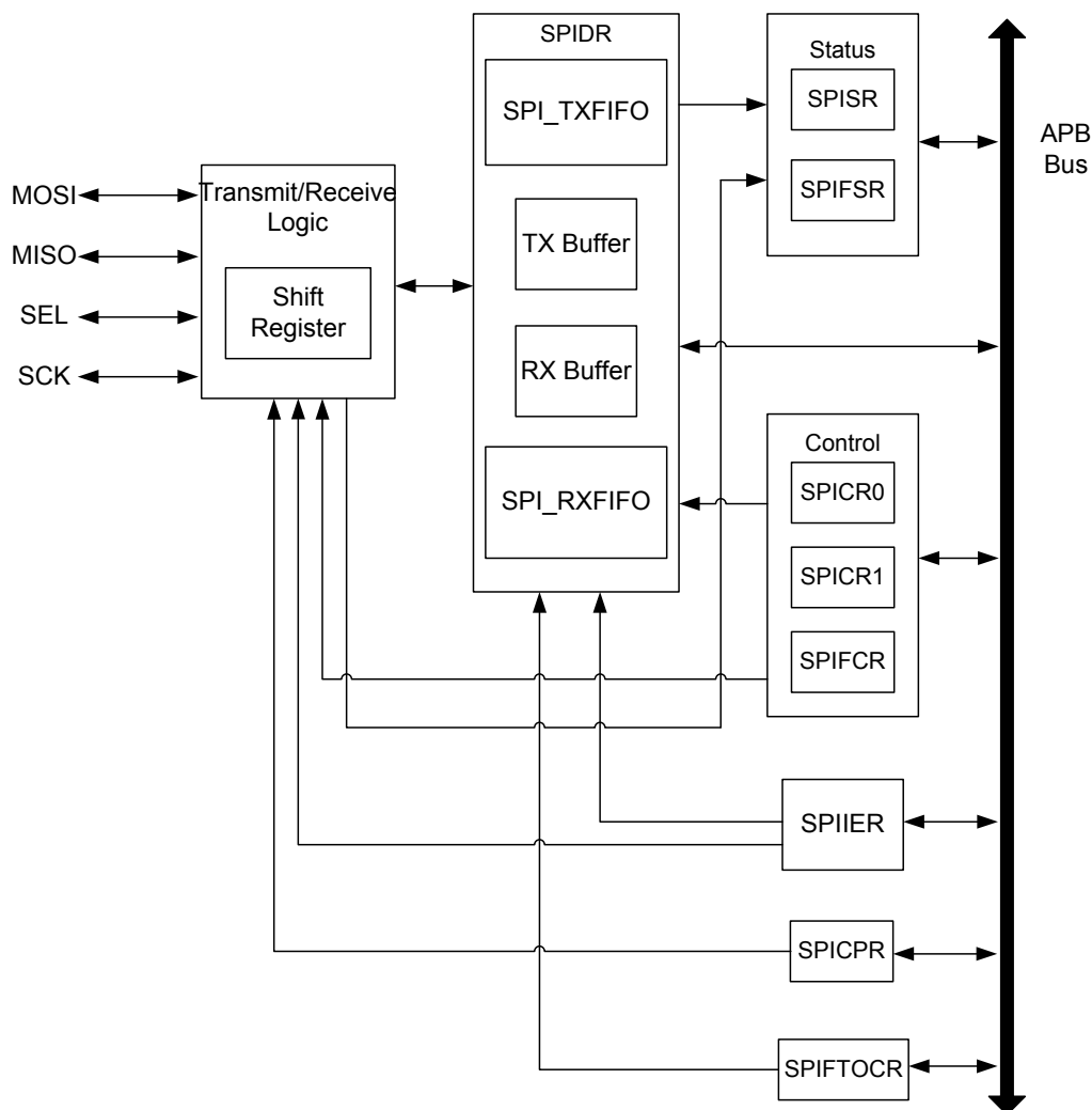
Figure 146. SPI Block Diagram
