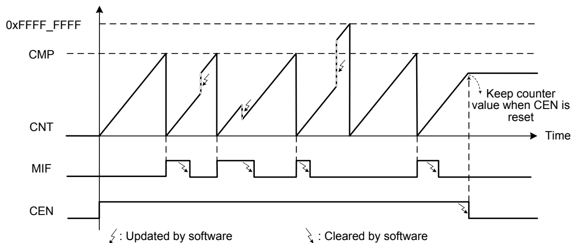
Figure 66. BFTM – Repetitive Mode
