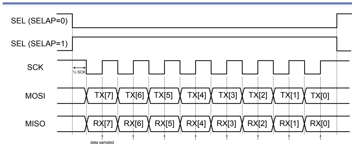
Figure 153. SPI Single Byte Transfer Timing Diagram – CPOL = 1, CPHA = 1
