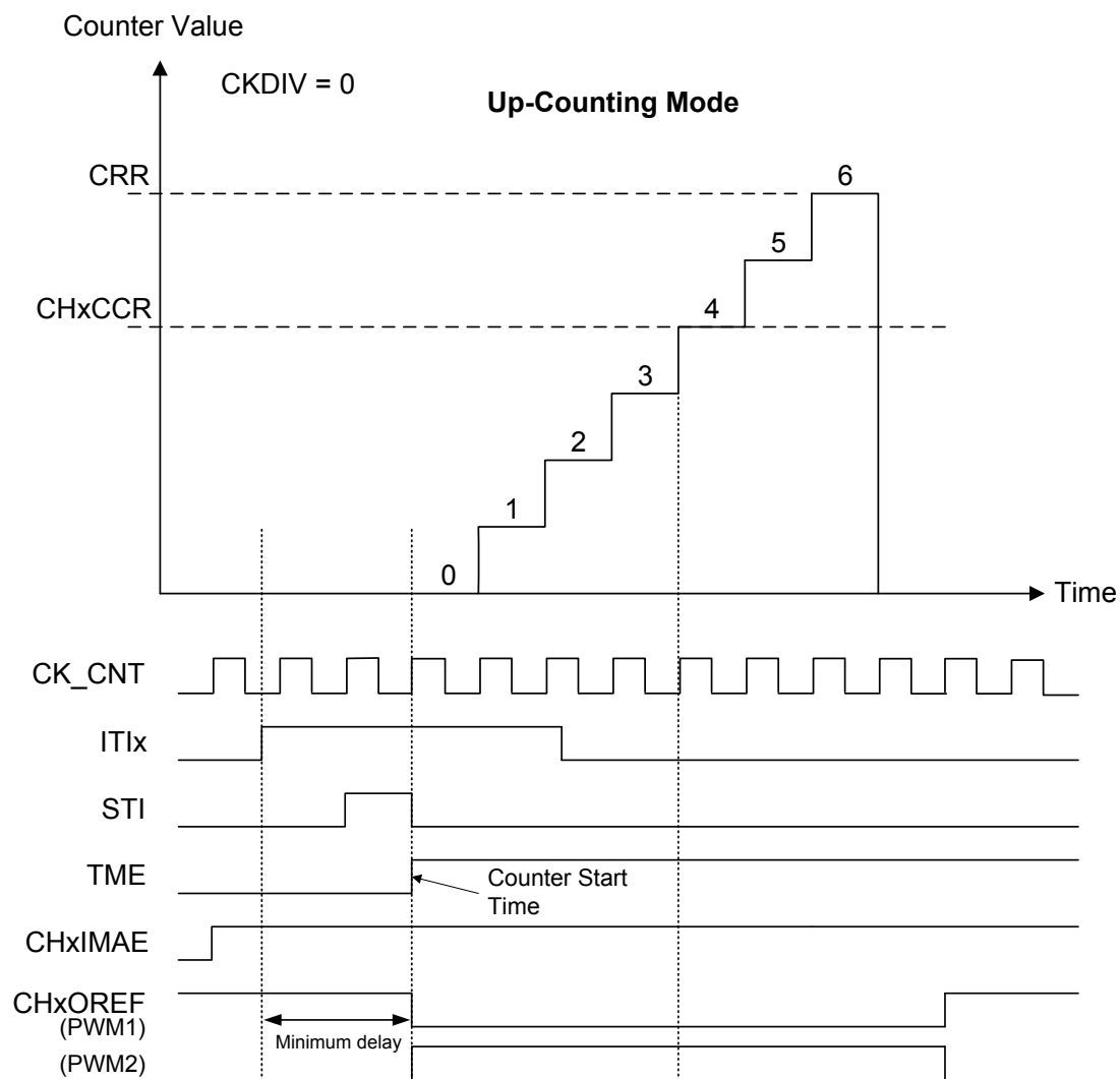
Figure 105. Immediate Active Mode Minimum Delay
