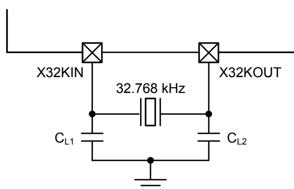
Figure 17. External Crystal, Ceramic, and Resonators for LSE
