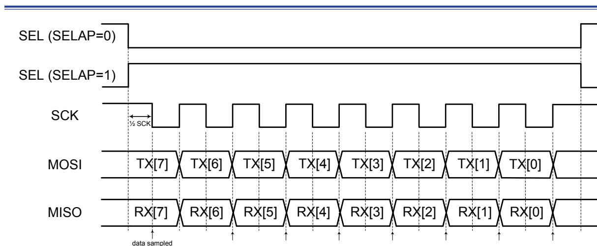
Figure 151. SPI Single Byte Transfer Timing Diagram – CPOL = 1, CPHA = 0
