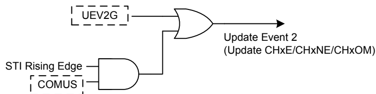
Figure 103. Update Event 2 Setup Diagram
