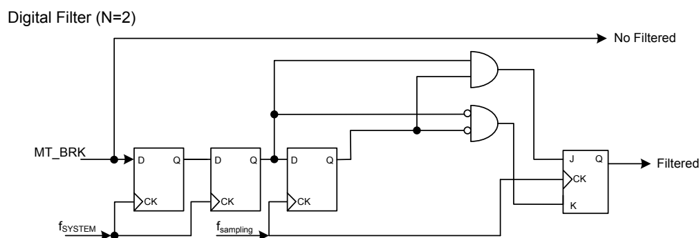
Figure 96. MT_BRK Pin Digital Filter Diagram with N = 2
