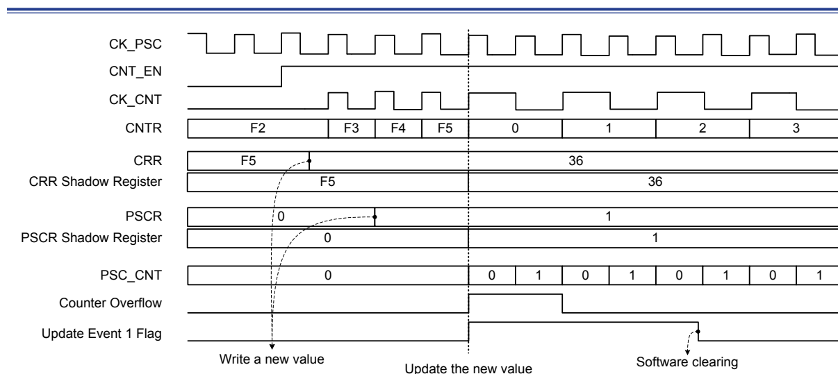
Figure 70. Up-counting Example
