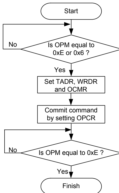
Figure 10. Word Programming Operation Flowchart
