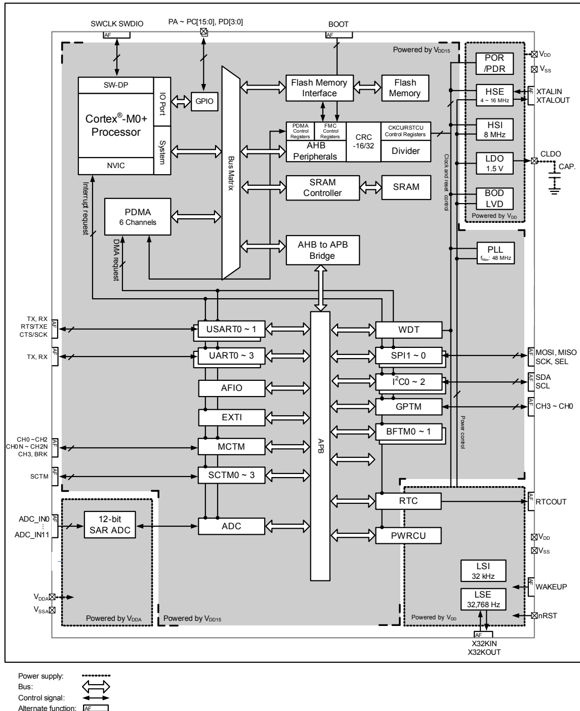
Figure 1. Block Diagram
