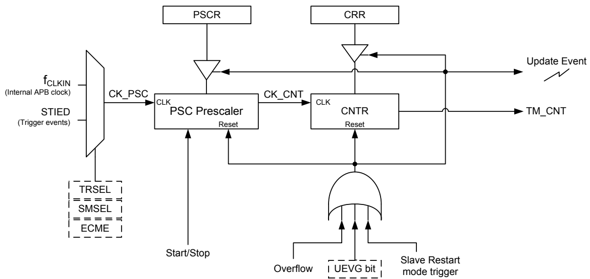
Figure 114. SCTM Clock Selection Source
