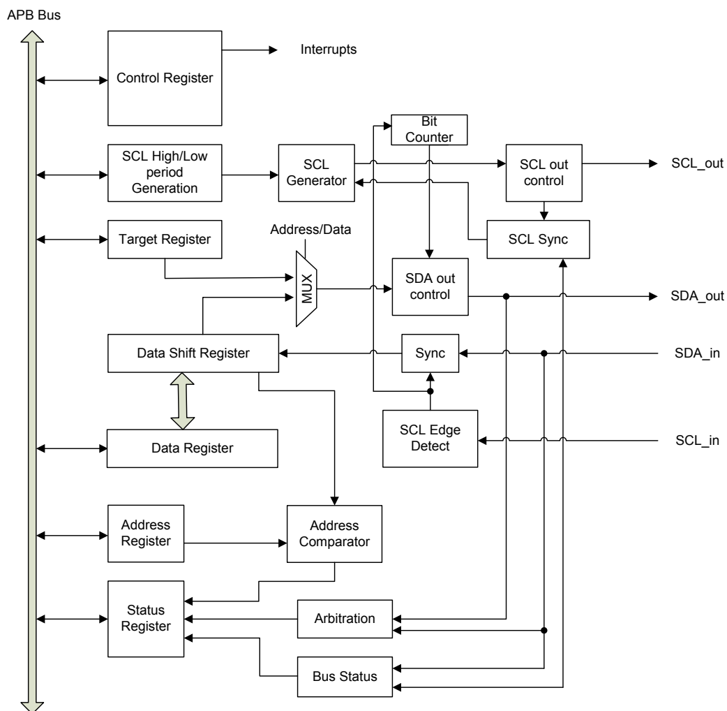
Figure 132. I 2 C Module Block Diagram
