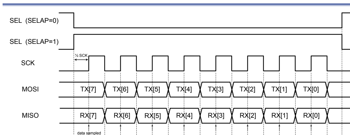
Figure 147. SPI Single Byte Transfer Timing Diagram – CPOL = 0, CPHA = 0
