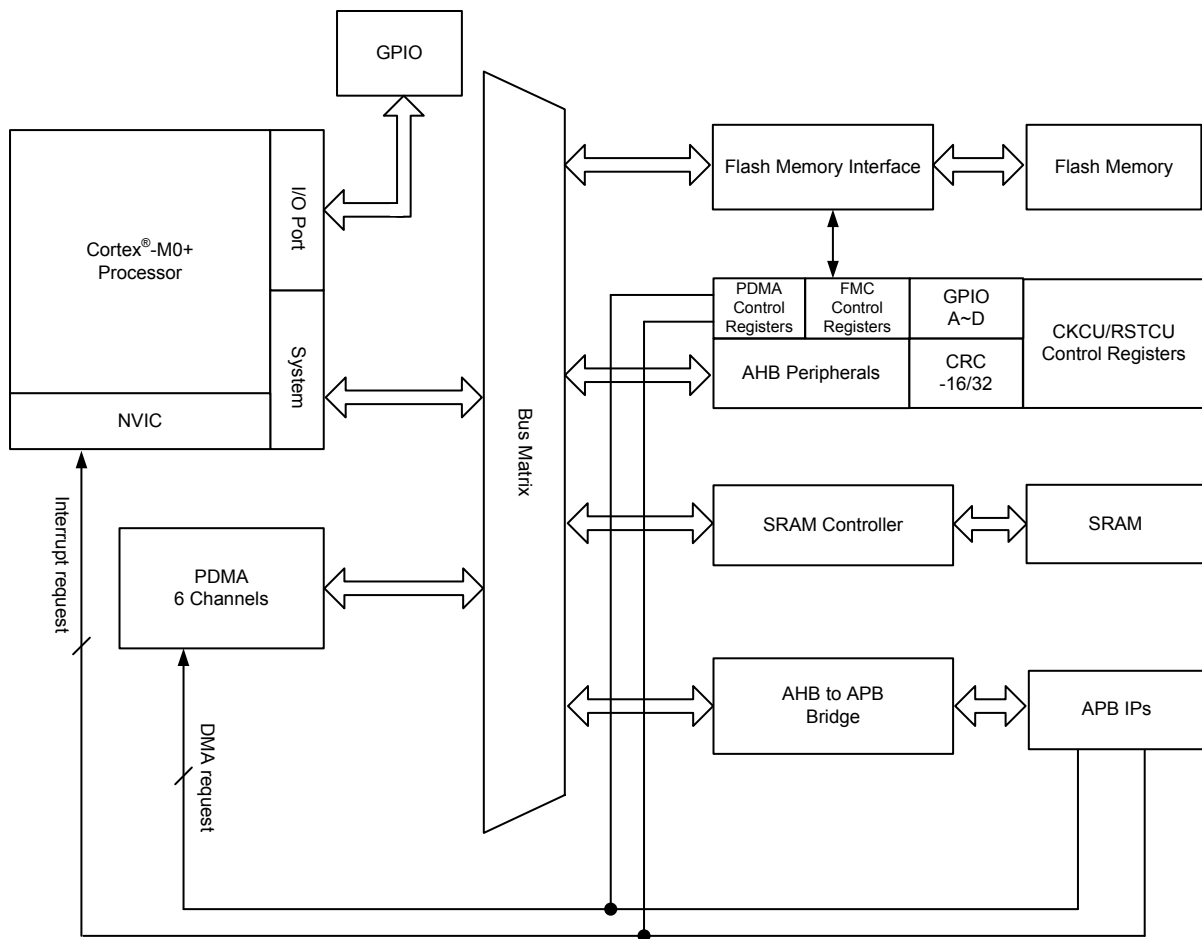
Figure 3. Bus Architecture
