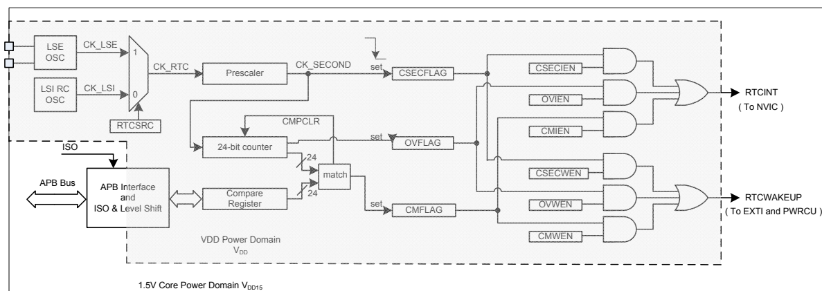
Figure 129. RTC Block Diagram
