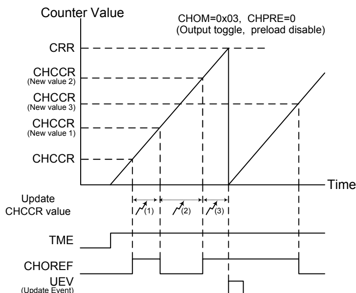
Figure 125. Toggle Mode Channel Output Reference Signal (CHPRE = 0)
