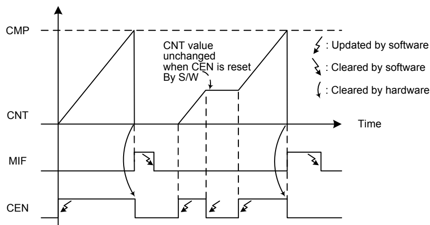
Figure 67. BFTM – One Shot Mode
