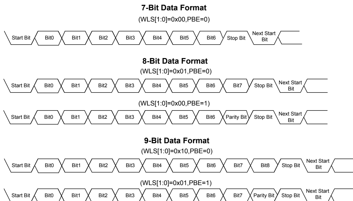
Figure 157. USART Serial Data Format
