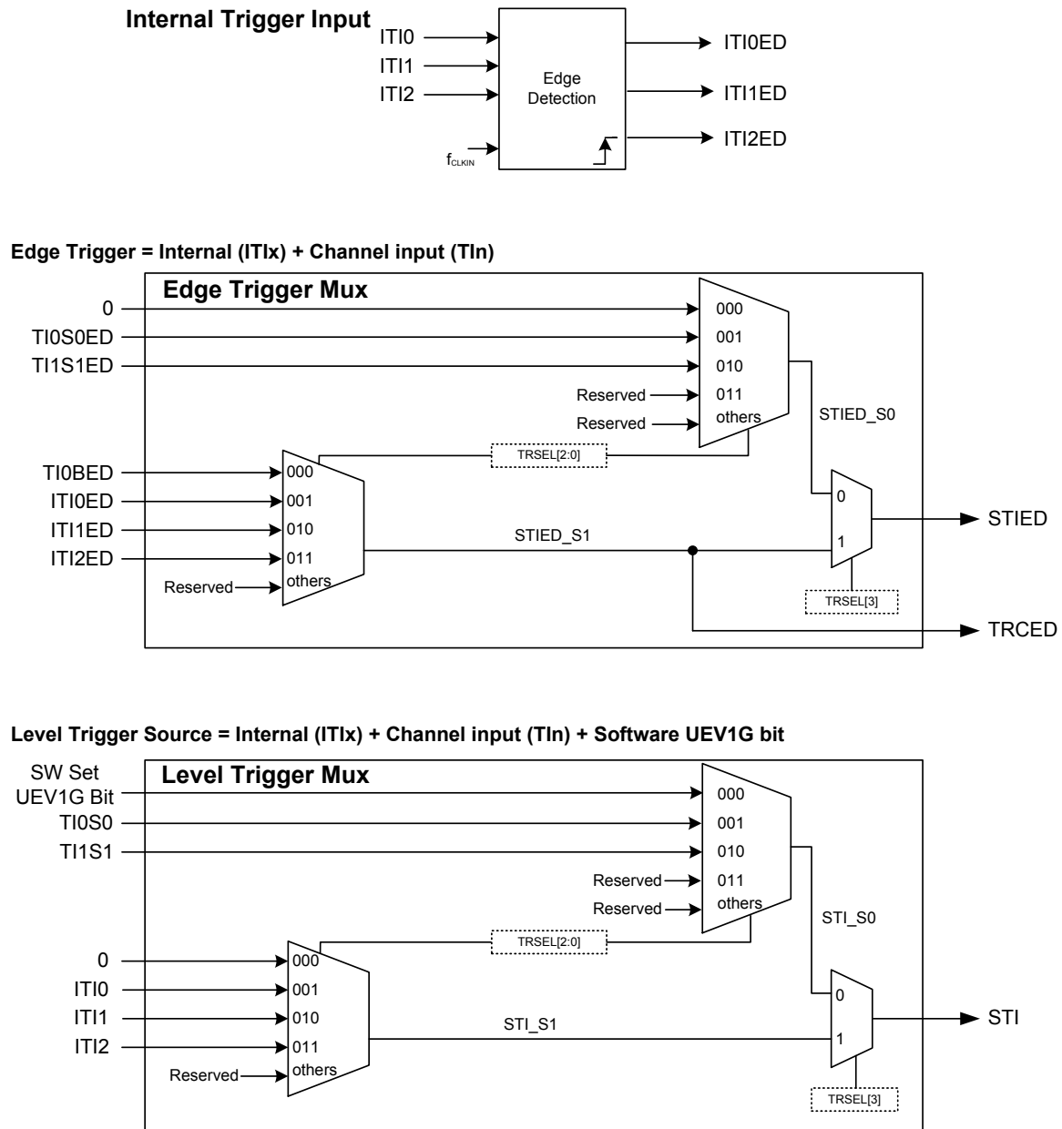
Figure 75. Trigger Controller Block
