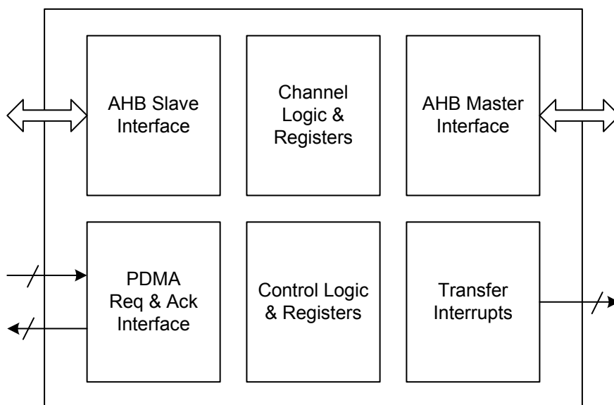
Figure 170. PDMA Block Diagram
