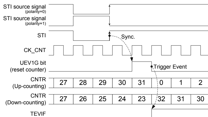
Figure 77. MCTM in Restart Mode
