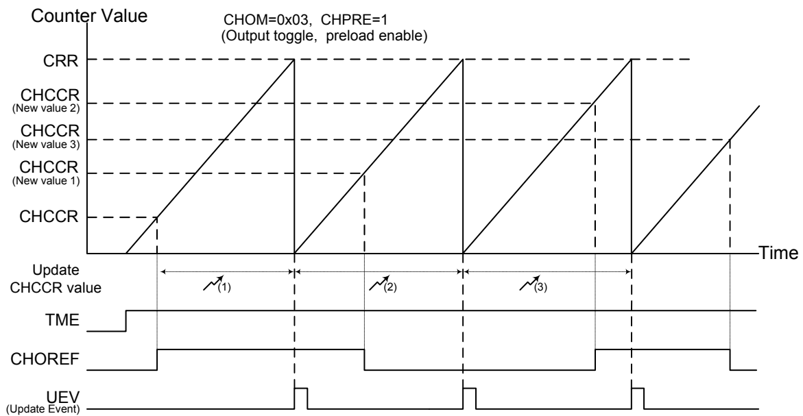
Figure 126. Toggle Mode Channel Output Reference Signal (CHPRE = 1)
