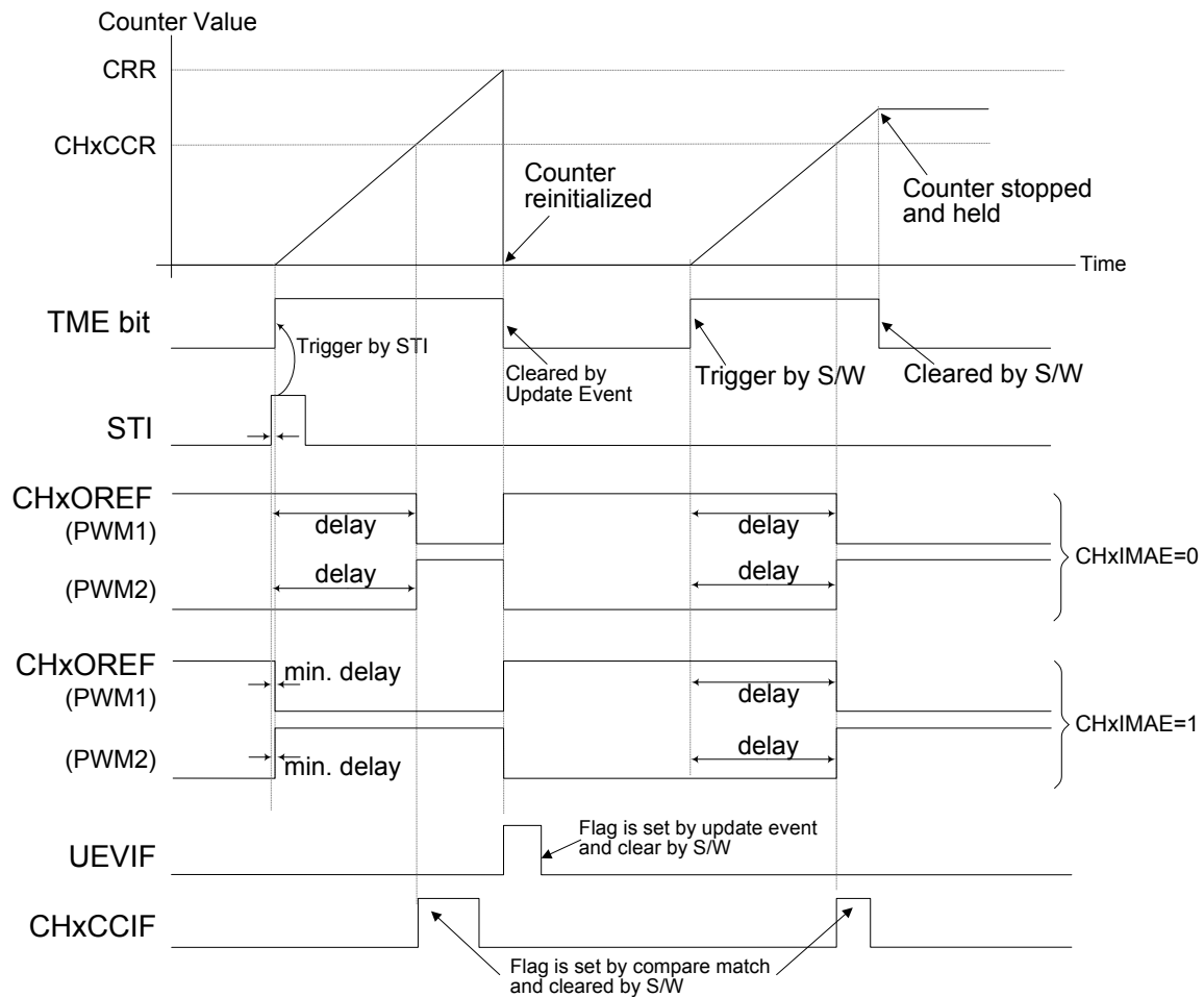
Figure 58. Single Pulse Mode
