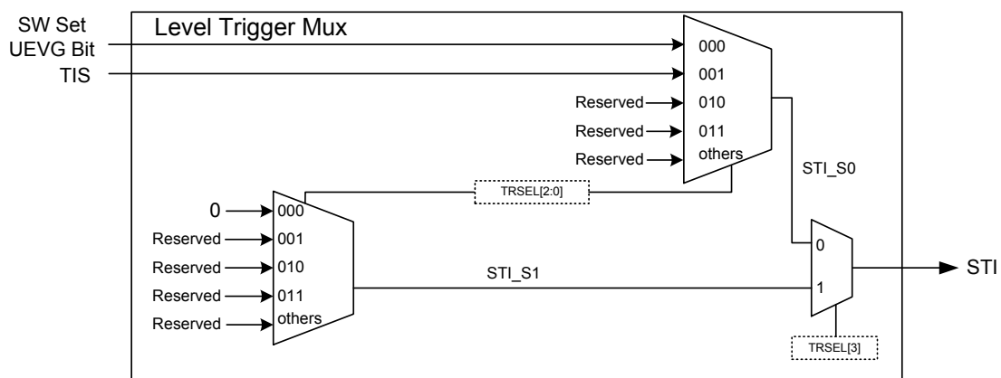
Figure 115. Trigger Control Block
