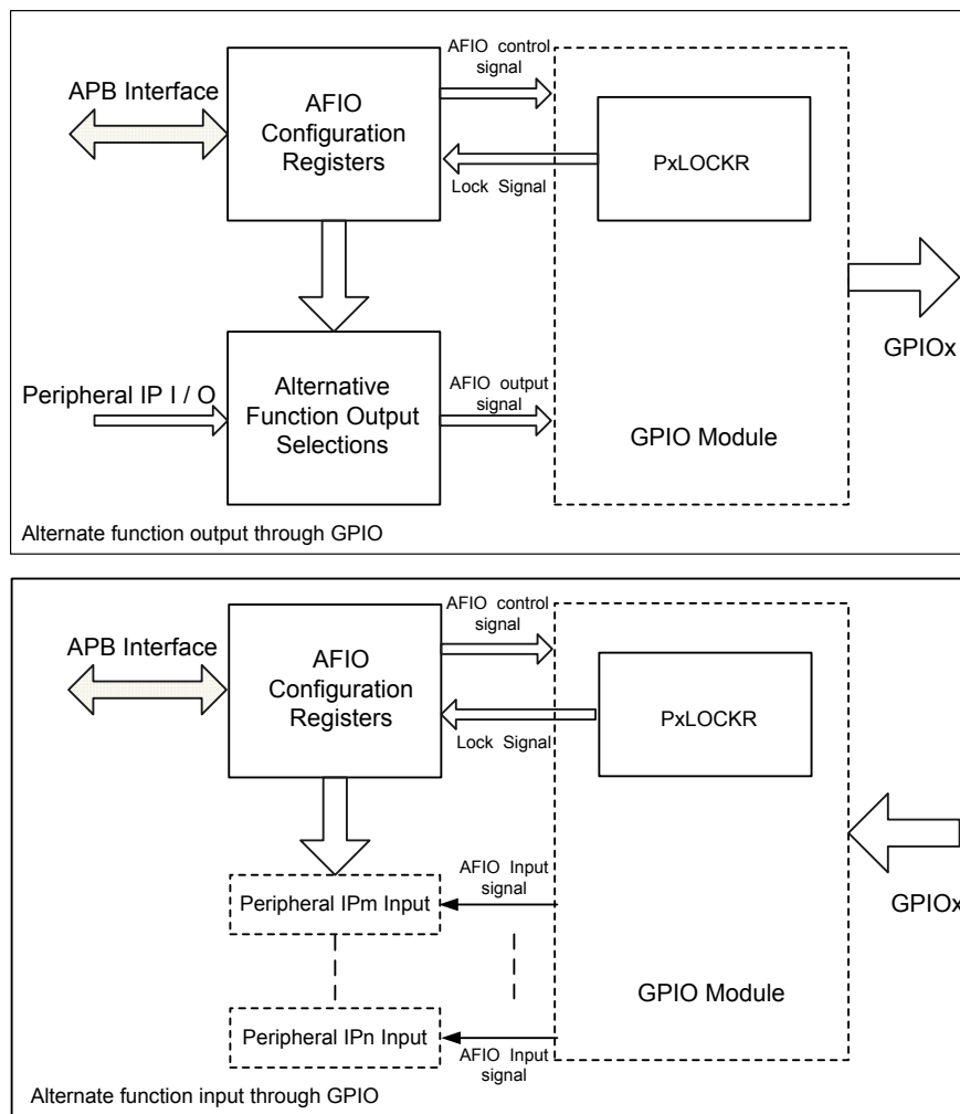
Figure 22. AFIO Block Diagram
