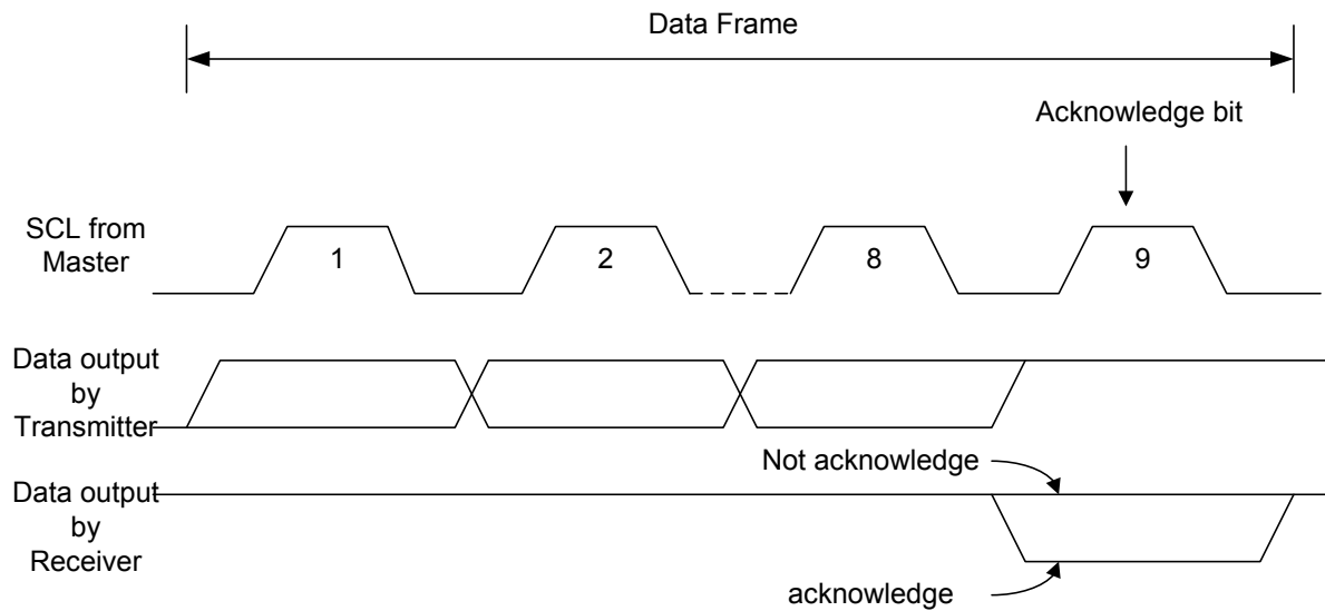
Figure 138. I 2 C Bus Acknowledge
