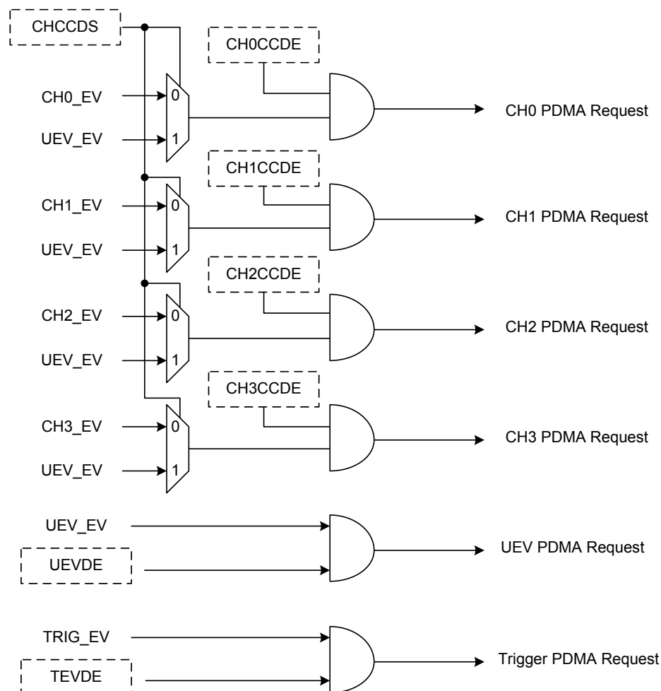
Figure 64. GPTM PDMA Mapping Diagram
