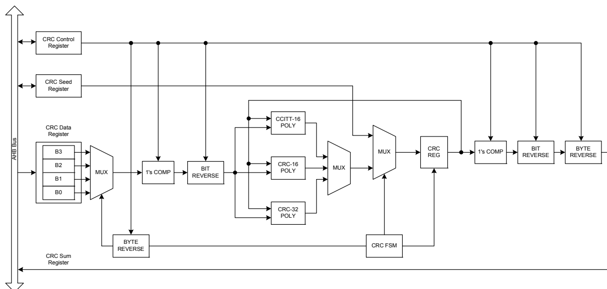
Figure 173. CRC Block Diagram
