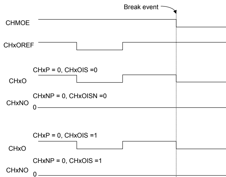
Figure 100. Hardware Protection When Both CHxO and CHxNO are in Active Condition
