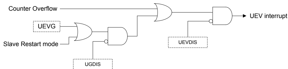
Figure 128. Update Event Setting Diagram
