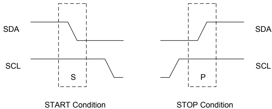
Figure 133. START and STOP Condition
